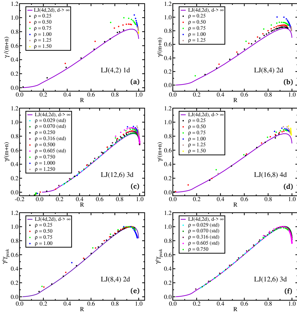
Figure 3: (R, \gamma) diagrams for the LJ(4d, 2d) potential for d = 1, 2, 3, 4 . The density range is given in the inset while the temperature varies from T = 0.5 \rightarrow 5 in 0.5 steps (except when otherwise stated). The virial approximation curve Eq. (13) for n = X = 2 is represented by the full violet curve. (a) d = 1 , the potential is v_{4,2}(r) . (b) d = 2 , the potential is v_{8,4}(r) . Here the temperature steps are 0.25 starting from T = 0.25 . For \rho = 0.25 and \rho = 0.50 , the highest temperature simulated is T = 12.00 and T = 7.00 , respectively. This ensures visibility of the peak in \gamma(R) in panels (e) and (f). (c) d = 3 , the potential is v_{12,6}(r) . Data for both the standard 12-6 LJ (labelled "std") and the generalized LJ(12,6) are presented. The unit length for these two potentials is different, resulting in different definitions for the density. The lowest temperature on each isochore is either along the liquid-gas or liquid-solid coexistence curves for the standard LJ; for the generalized LJ(12,6) densities and temperatures are the same as in (a) with the addition of T = 0.25, 0.75 . The standard LJ phase diagram is therefore explored more comprehensively: the highest temperature on each isochore is roughly 200 times the lowest, well above T = 5 . Thus we recover the IPL limit (R, \gamma) \rightarrow (1, 4) . The similarity between panels (a),(b), and (d) demonstrates that covering such a wide region of the phase diagram is not necessary to get an almost complete \gamma(R) curve. (d) d = 4 , the potential is v_{16,8}(r) . (e) and (f) correspond, respectively, to panels (b) and (c) where for each isochore the density-scaling exponent \gamma is scaled by its peak value \gamma_{\text{peak}} . The value of \gamma_{\text{peak}} is different on each isochore.
