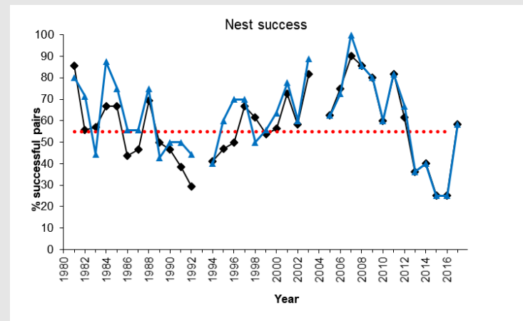
Figure 2: Nest success- proportion of occupied historical/“known” sites that produced young; black line is all sites, blue line is comparable “monitoring sites” only (smaller sample size 1981-2002). The red line is the threshold where there “would be cause for concern in the short term” (USFWS 2003).
