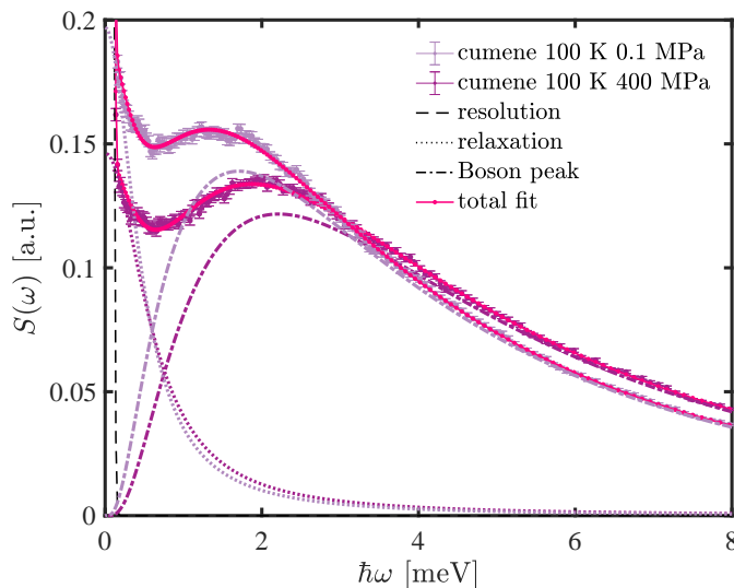
Figure 8.20: Fit to cumene spectra at 100 K, 0.1 MPa and 400 MPa: a sum of a Lorentzian relaxation and a log-normal function to fit the Boson peak. The amplitude of the fast relaxation from the fit is three orders of magnitude smaller than the elastic peak intensity.
