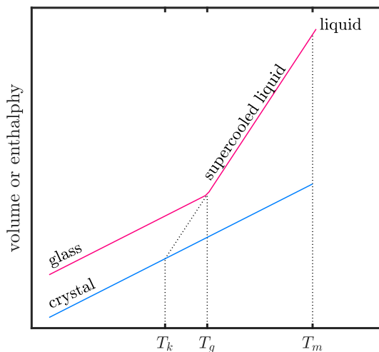
Figure 2.1: A sketch of volume or enthalpy change upon cooling from the liquid state into the supercooled liquid and the glass, or into the crystal state. An abrupt change in enthalpy as a function of temperature is observed at the transition from liquid to crystal state.
