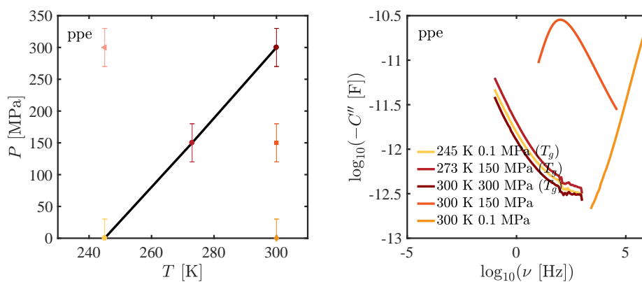
Figure 8.5: Left: Phase diagram of state points in temperature and pressure that are studied in this section on PPE from IN5. The black line is the glass transition isochrone found from dielectrics. Right: Imaginary part of capacitance from state points shown to the left.
