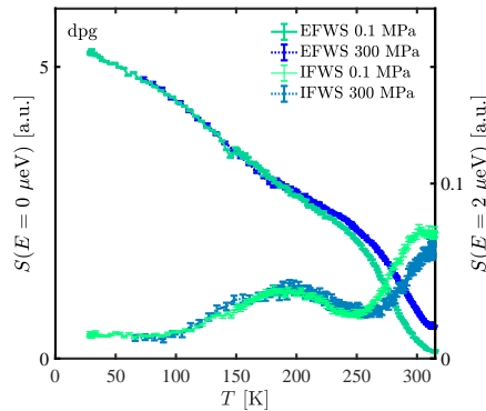
Figure 7.6: FWS from IN16B on DPG as a function of temperature at ambient pressure and 300 MPa. The pressure-dependent alpha relaxation is observed to enter the instrument window at around 300 K, while the pressure-independent methyl-group rotation is visible over a broad temperature range with a maximum at roughly 200 K.
