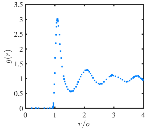
Figure 4.1: Sketch of the radial distribution function, g(\mathbf{r}) , of an amorphous system. Peaks are seen for values of \mathbf{r}/\sigma corresponding to first, second, etc. coordination shell in a liquid with molecules of size \sigma .
