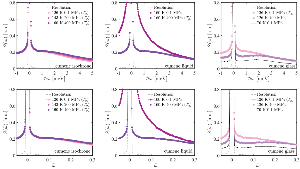
Figure 8.3: Comparison of the cumene spectra as a function of energy transfer plotted as a function of energy on absolute scale and in reduced units.
