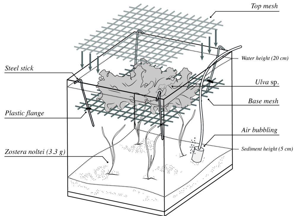
Fig 1. Aquarium set-up.
