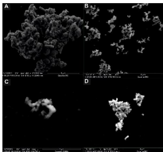
Fig. 2 SEM images of 0.01 \mu\text{m} filters with the example of most commonly observed colloids: A) Fe-Sb-Si-S phases, Beaver Brook B) Fe-As-Si-S-Ca phases, Poproč Agnes adit; C) Fe-Si-S phases, Medzibrod D) Fe-As-Si-Ca phases Poproč SN
