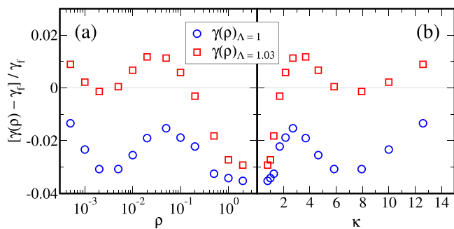
FIG. 7. Relative difference between the estimated \gamma(\rho) (Eq. (27)) and \gamma calculated from the equilibrium fluctuations via Eq. (13) (denoted in the figure by \gamma_f ). The prediction \gamma(\rho)_{\Lambda=1.03} is generally in best agreement with the values from the equilibrium fluctuations.
