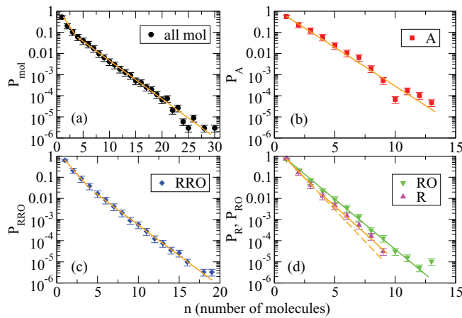
FIG. 3. (a) Probability P_{\text{mol}}(n) of having a nanoaggregate containing n aromatic molecules versus n . (b) Probability P_A(n) of having a nanoaggregate containing n asphaltene molecules versus n . (c) Probability P_{\text{RRO}}(n) of having a nanoaggregate containing n resin or resinous oil molecules versus n . (d) Probability P_R(n) of having a nanoaggregate containing n resin molecules versus n and probability P_{\text{RO}} of having a nanoaggregate containing n resinous oil molecules versus n . In every case the straight lines (orange or green) are guides to the eye. They highlight the monoexponential behavior in (b) and (d), when resinous oil molecules are counted, and the biexponential behavior in (a)–(d), when resin molecules are counted. The error bars correspond to the standard deviation estimated from eight independent simulations.
