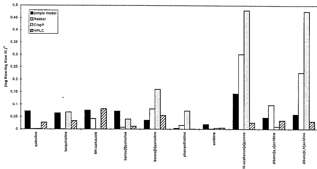
Fig 7.2. Squared errors in \log K_{ow} for azaarenes using the best simple specific model, Rekker and Mannholds aromatic f-fragment method, ClogP or HPLC (Diol-35-1) for predictions.
