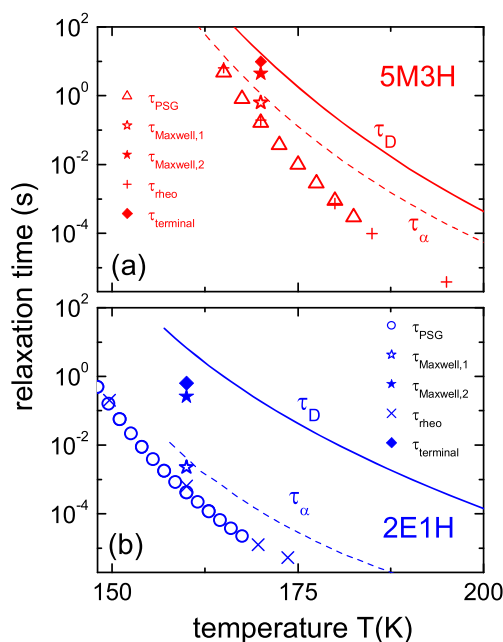
Fig. 3 Temperature-dependent shear relaxation times of a 5M3H ( red triangles : PSG technique, current work; red crosses : rheometer, current work) and b 2E1H ( blue circles and blue crosses , taken from ref. 15). The diamonds reflect the time scales of the terminal relaxation modes indicated by the arrows in Fig. 2b. The stars are calculations based on the Maxwell relation: the open symbols refer to \tau_{\text{Maxwell},1} = \eta_0/G_\infty and the filled symbols to \tau_{\text{Maxwell},2} = \eta_0/G_{\infty,\text{supra}} , respectively. The lines represent dielectric time constants for the \alpha process ( dashed lines ) and for the Debye process ( solid lines ) taken from Refs. 25 6
