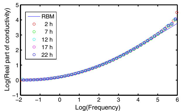
FIG. 3 (color online). Real part of \sigma(\omega)/\sigma(0) plotted as a function of empirically scaled frequency for CKN annealed at 308 K. The figure shows data taken 2, 7, 12, 17, and 22 hours after the glass transition. No shape change is observed. The full curve is the prediction of the random barrier model (RBM), Eq. (2).
