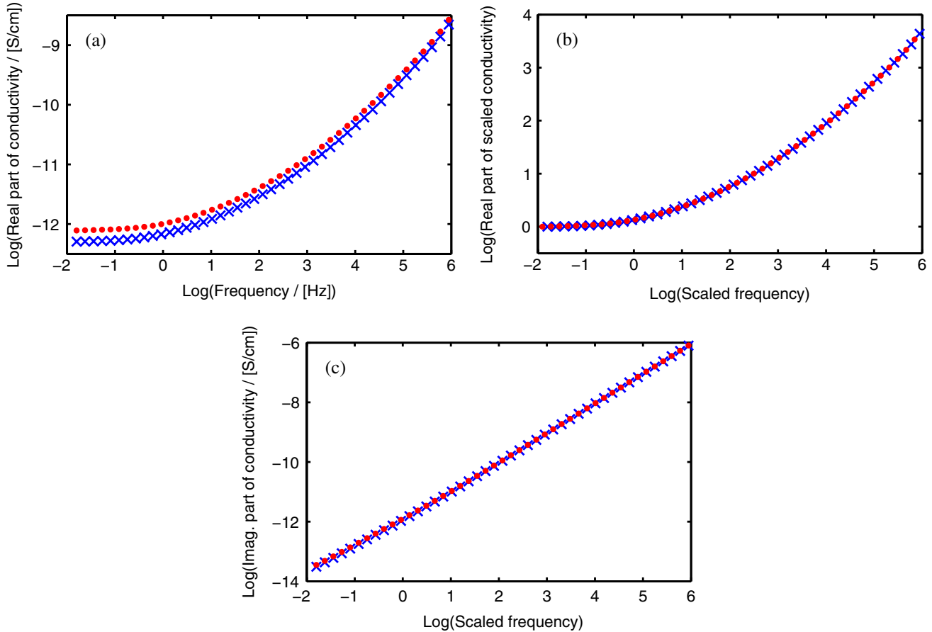
FIG. 2 (color online). (a) Alternative representation of the data of Fig. 1, showing the real part of the ac conductivity \sigma(\omega) of CKN annealed at 308 K two hours after the glass transition (red dots) and 22 hours after (blue crosses). Annealing decreases the conductivity at all frequencies. (b) The real part of the scaled ac conductivity \sigma(\omega)/\sigma(0) two hours after the glass transition (red dots) and 22 hours after (blue crosses) plotted as a function of frequency scaled empirically to maximize the overlap. No shape change is observed. (c) The imaginary part of the conductivity two hours after the glass transition (red dots) and 22 hours after (blue crosses). Virtually no changes are observed, and for both data sets the imaginary part is almost proportional to frequency. These facts show that the major contribution to the imaginary part derives from the electronic polarization (which is instantaneous compared to the ionic motion), an observation that is key to understanding why the modulus peak narrows during annealing (Fig. 1).
