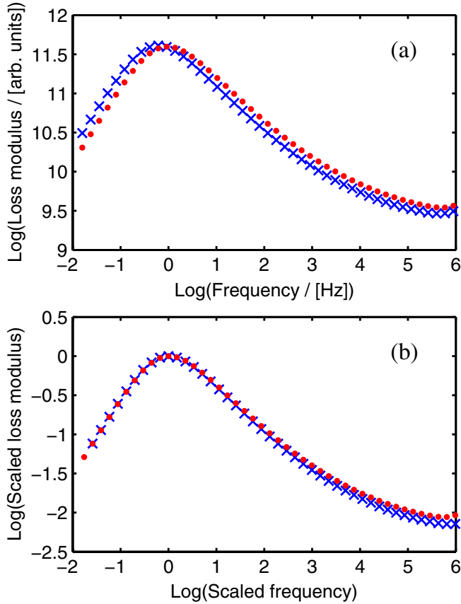
FIG. 1 (color online). (a) Log-log plot (base 10) of the loss modulus of CKN annealed at 308 K. The figure shows data obtained two hours after cooling to 308 K at a rate of 10–15 K/min from above the glass transition at 335 K (red dots), as well as 22 hours after cooling to 308 K (blue crosses) (data from Ref. [5]). (b) The same data plotted by scaling with the modulus maximum and the corresponding frequency. The modulus peak narrows upon annealing.
