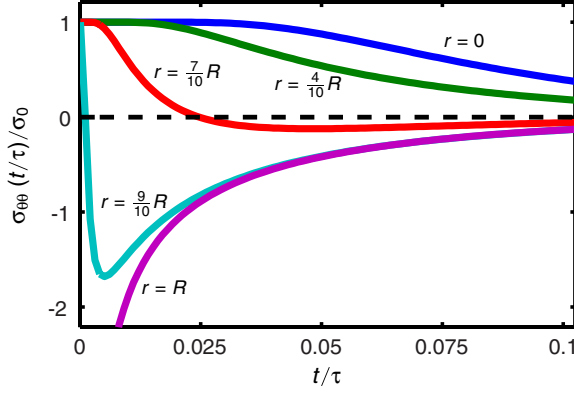
FIG. 5. The \theta\theta component of the stress tensor, 1 - \frac{3}{2}F_2 + \frac{1}{2}F_1 , as a function of time scaled with the initial stress \sigma_0 . There is an initial adiabatic positive step up in \sigma_{\theta\theta} throughout the sphere. The regions that have been reached by the incoming diffusive heat at a certain point in time experience a negative \theta\theta -stress component since the inner unheated regions pull the outer heated regions inwards.
