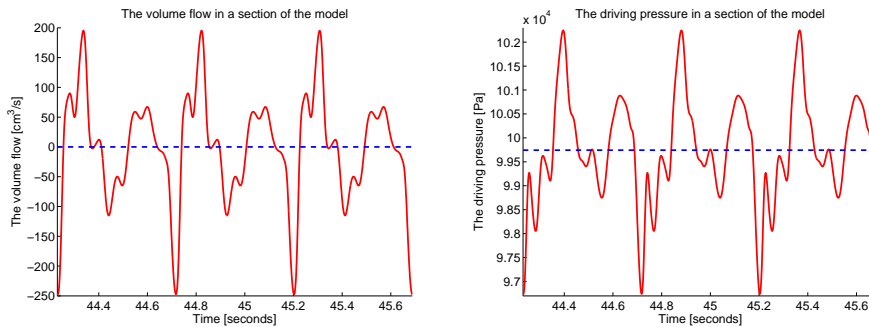
Figure 5.3: Three periods of a numerical test of the model with the number of sections N = 50 and the three sections pinching site centered at section 13, midway on the soft tube. Model setup as defined in section 5.2. Both flow and pressure oscillations are very dramatic, while mean flow is almost zero, 1.67 \cdot 10^{-4} \text{ cm}^3/\text{s} , and mean pressure drops a little compared to atmospheric pressure, 9.97 \cdot 10^4 \text{ Pa} .
