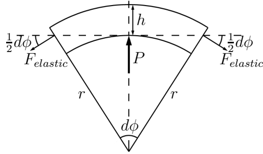
Figure 3.3: The force from the pressure is normal to the tube wall, but it is balanced by the sine-component of the elastic force in the wall.
