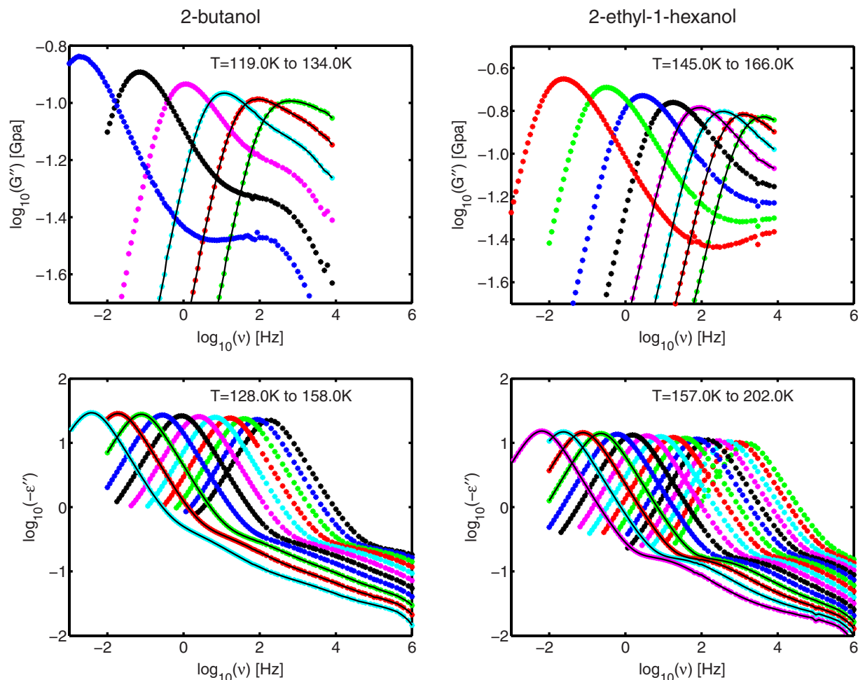
FIG. 1. (Color online) Selected dielectric and shear-mechanical spectra for the two liquids (the full data set is available online, see Ref. 29). Temperature intervals are indicated and the step size is 3 K. Temperatures that are highlighted by a full line through the points exist for both dielectric and shear-mechanical measurements, this is only the case in a limited temperature interval, where an overlap exists between the high temperature shear data and low temperature dielectric data. Top: shear-mechanical loss as function of frequency. Bottom: dielectric loss as function of frequency. To enhance readability of the figure, the dielectric spectra have been truncated at low frequencies, at around the onset of the contribution from conduction.
