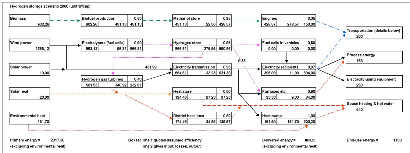
Figure 14. Danish 2060 scenario based on use of hydrogen storage without fuel cells.
