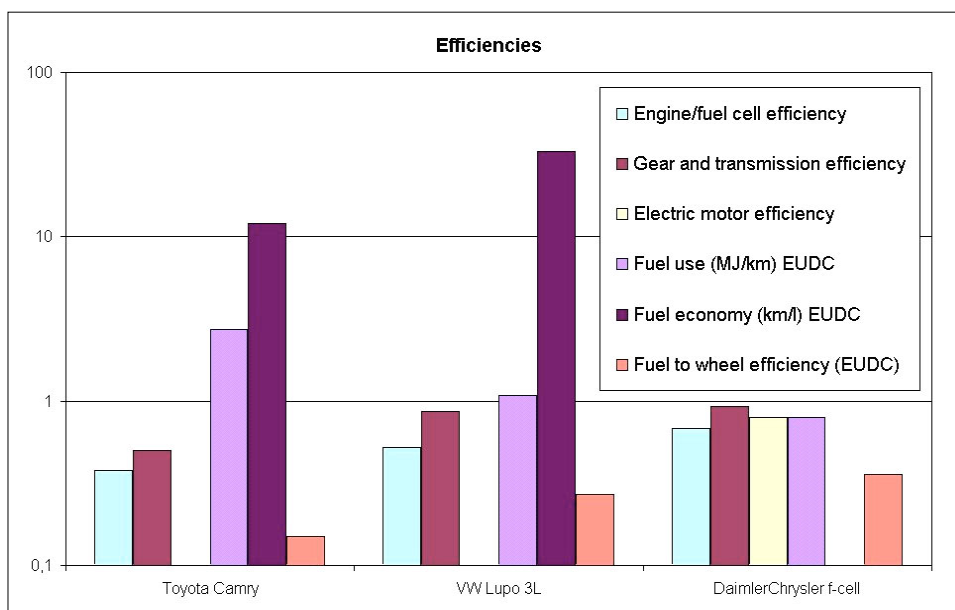
Figure 8. Comparison of contributions to and total efficiency of the three cars studied in the LCA analysis (1). As indicated in the insert, two columns carry three dimensions, while the rest are dimensionless efficiencies. The first f-cell cars demonstrated in Japan and Australia during mid-2004 has an 80% higher fuel use than indicated here.
