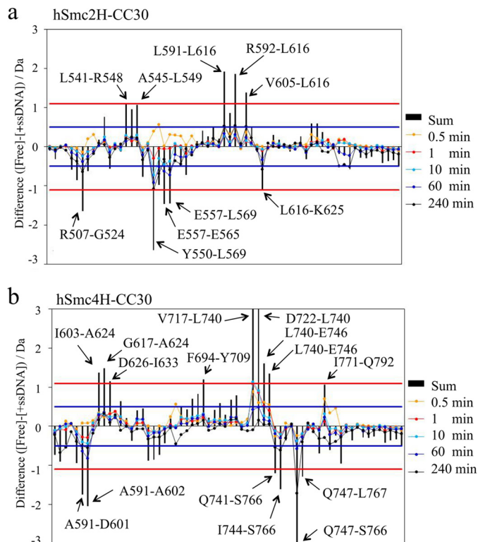
FIGURE 7. Differential map of the hSmc2–4 hinge with middle coiled coils. For each peptide, the deuterium uptake at each exposure time of hSmc2–4 hinge with middle coiled coils in the presence of ssDNA (+ssDNA) was subtracted from that in the absence of ssDNA (Free). The summation of changes in the uptake over all exposure times has also been indicated. Positive or negative values indicate that the uptake rates were reduced or enhanced, respectively, upon interaction with ssDNA. Red lines, when the sum of difference is over 1.1 Da between two states for a peptide, the result reflects differing amide proton environments of the region covered by the peptide in solution, with 98% confidence. Blue lines, a difference of over 0.5 Da (at a specific exposure time) in a peptide indicates the differing amide proton environments of the region. a , hSmc2H-CC30 in the heterodimer. b , hSmc4H-CC30 in the heterodimer.
