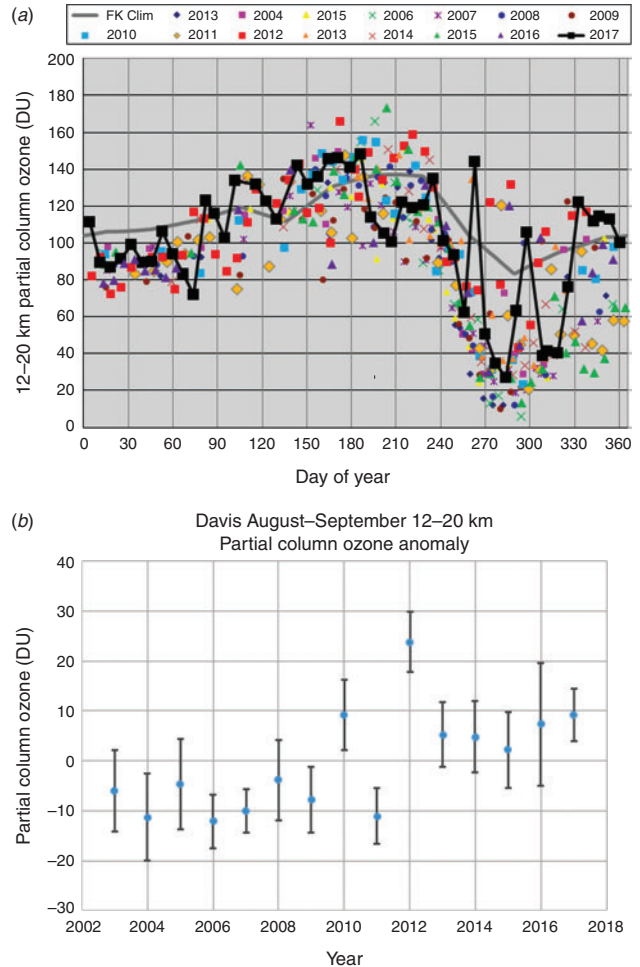
Fig. A1.3. Time series of partial column ozone for the height interval 12–20 km obtained from ozonesonde measurements at Davis, Antarctica (68.6°S and 78.0°E). (a) Annual data for all years of measurement, with data for 2017 highlighted with black filled squares and solid line. The grey line is a climatological mean from Fortuin and Kelder (1998) interpolated to the location of Davis. Note that at Davis, this height range is almost exclusively above the lapse rate tropopause and generally below the burst height of the ozonesonde balloons in winter. (b) Average 12–20 km partial column ozone anomaly over August and September (days 213–273 in nonleap years) for 2003–17 (see text for details of the calculation method). The vertical bars span a range of twice the standard error in the mean.
