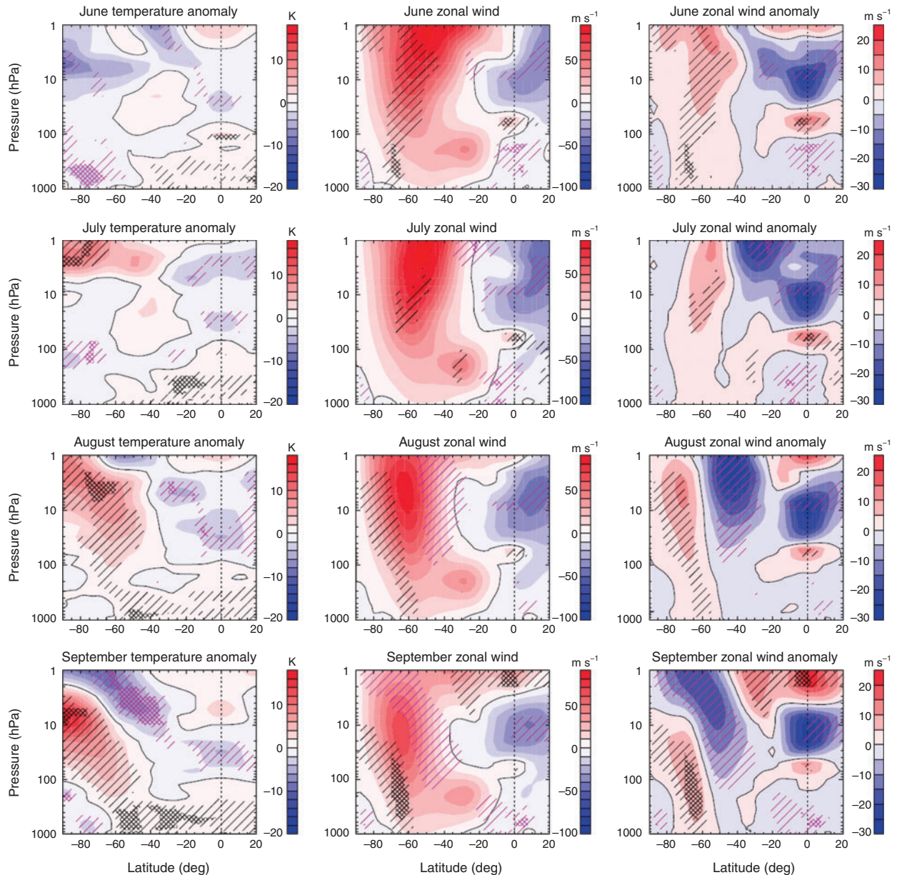
Fig. 4. Pressure-latitude cross sections from 90°S to 20°N of monthly mean ERA-Interim reanalysis parameters for (from top row to bottom row) June, July, August and September 2017. (Left column) Temperature anomaly with respect to the 1979–2016 climatology. (Middle column) Zonal wind speed. (Right column) Zonal wind speed anomaly with respect to the climatology. The zero contour is highlighted in black. Single magenta (black) diagonal hatching denotes values below (above) the interdecile range over the climatology; magenta (black) crossed diagonal hatching denotes values below the minimum (above the maximum) of the climatology. The vertical dotted line marks the location of the equator. Note that the cross sections poleward of 65°S and for pressures greater than ~700 hPa may be within the topographical surface.
