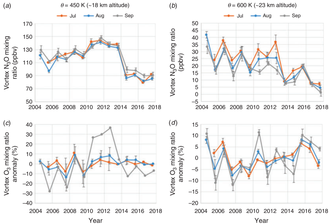
Fig. 12. Vortex-average monthly mean (top row) nitrous oxide (N 2 O) mixing ratio and (bottom row) ozone (O 3 ) mixing ratio anomaly (with respect to the average over all available years) for isentropic levels of (left column) 450 and (right column) 600 K for (orange line and filled circles) July, (blue line and filled circles) August and (grey line and filled circles) September. The vertical bars denote \pm 1 standard deviation in the daily means over each month; the standard deviation for ozone in September at \theta = 450 K is not shown for clarity but has an average value of 39%. The panels were produced from Aura/MLS v4.2 pressure-level measurements of N 2 O and O 3 (which were selected according to criteria described in version 4.2-3.0 of https://mls.jpl.nasa.gov/data/v4-2_data_quality_document.pdf , accessed 1 May 2020). The measurements were interpolated to isentropic levels and spatially averaged within the ‘inner vortex edge’ region using the MLS Derived Meteorological Product data set based on MERRA-2 reanalysis. As noted by Manney et al. (2007), identification of the vortex edge can be problematic under certain circumstances, particularly outside of winter, and so the values presented may not necessarily accurately reflect the broad average of the inner vortex.
