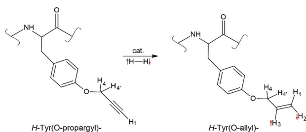
Figure 5. PHIP of peptides by hydrogenation of a side chain (PHIP-label). In this example, a propargyl moiety was added to tyrosine in a peptide. The addition of pH_2 results in hydrogenation of propargyltyrosine to yield a hyperpolarized allyltyrosine peptide. In the sunflower trypsin inhibitor SFTI-1, polarizations of P(^1H) = 9.6\% [67] were obtained in the allyl product (right).
