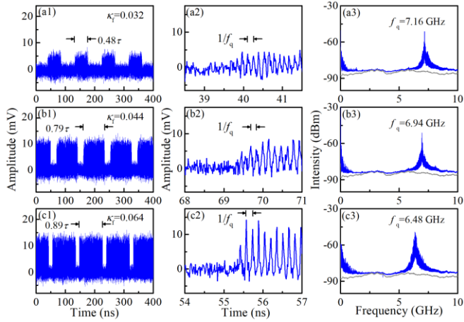
Fig. 3. Switching between steady state and quasi-periodic state at feedback strength of \kappa_f = 0.032, 0.044 and 0.064 , from top to bottom, with the bias current of I = 4I_{th} . From left to right, columns 1 and 2 are temporal waveforms on different time scale, and column 3 lists electrical spectra.
