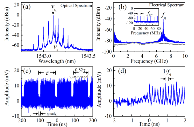
Fig. 2. Switching between steady state and quasi-periodic state at I = 4I_{th} , \kappa_f = 0.056 : (a) optical spectrum, (b) electrical spectrum, (c) and (d) intensity waveforms on different time scales.
