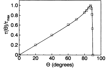
FIG. 3. Points selected from the normalized torque data of Ref. 4 on Bi:2212 at B=1 and T=77.5 \text{ K} (squares) compared with the prediction of the 2D theory (solid line): Eq. (2) using M' (see text).
