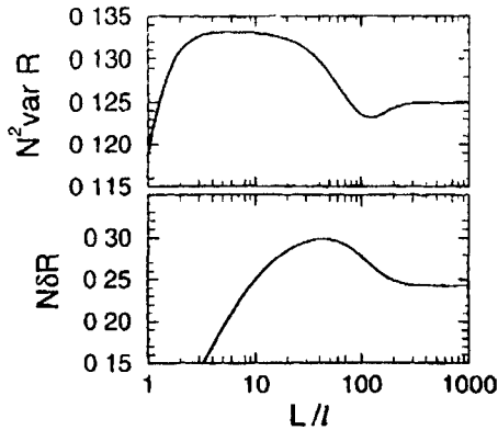
FIG 1 Length dependence of N \delta R and N^2 \text{var } R for \beta=1 and \gamma=10^{-4} , according to Eqs (5) and (6), in the regime \gamma N^2 \gg 1 . The variance \text{var } R of the reflectance crosses over from a plateau at 2/15N^2 (one dimensional limit) to a plateau at 1/8N^2 (zero dimensional limit). The crossover is nonmonotonic and occurs when the length of the waveguide becomes comparable to the decay length \xi=70 l of the transmittance. The weak-localization correction \delta R shows a similar crossover from 1/3N to 1/4N , but the plateaus are less well defined for this value of \gamma .
