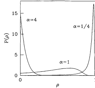
FIG. 1. Distribution of the phase rigidity \rho for \alpha=1/4 , 1, and 4, computed from Eq. (9). The crossover from the orthogonal to unitary ensemble occurs when \alpha \approx 1 , and is associated with large fluctuations in \rho around its ensemble average.
