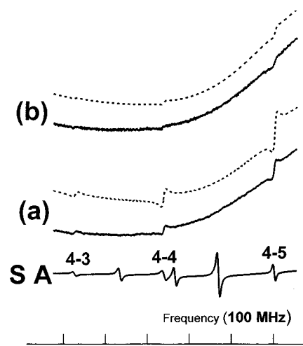
FIG. 1. Transmission spectrum through a thin Cs cell, as observed after demodulation of the applied FM. Full line spectra, experimental data with cell thickness (a) 10 \mu\text{m} or (b) 50 \mu\text{m} ; the incident power is \sim 50 nW, the beam diameter is \sim 4 mm, and the various narrow lines are the hyperfine components of the 852-nm line 6S_{1/2}(F=4) - 6P_{3/2}\{F=3,4,5\} . The simultaneously recorded saturated absorption (SA) spectrum is a frequency reference. The dashed lines above experimental data (a) and (b) are calculated spectra, assuming that \gamma/ku_{\text{th}} = 50 , with L/\lambda = 10 and L/\lambda = 50 , respectively (for a Cs linewidth of 5 MHz and a Doppler width of \sim 250 MHz). Each unit of the horizontal frequency scale stands for 100 MHz.
