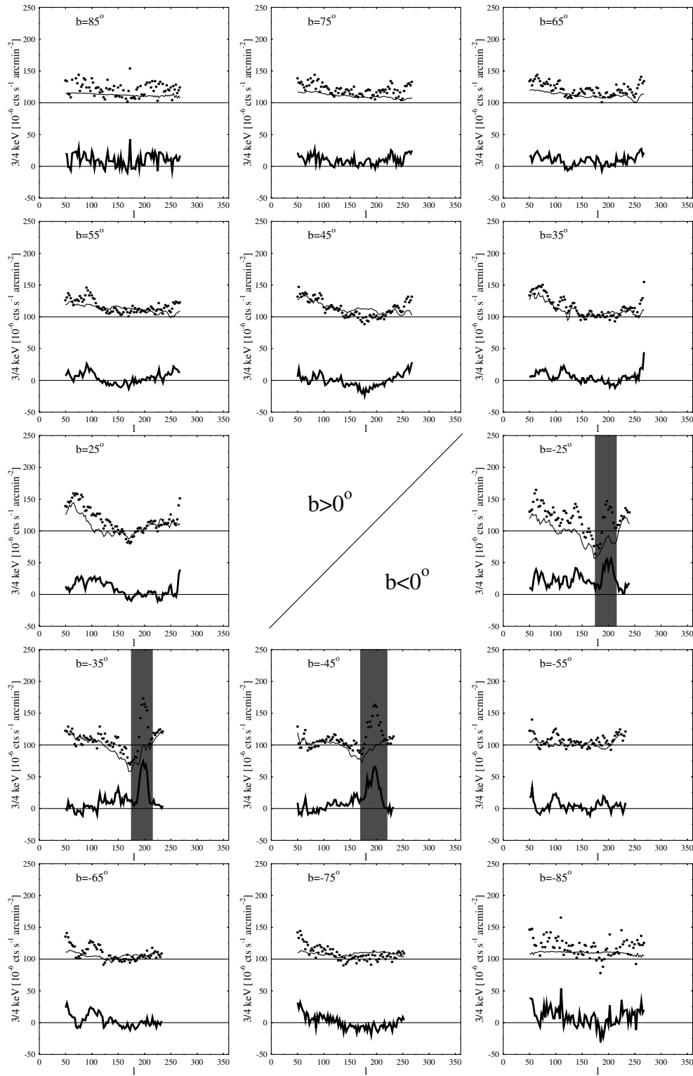
Fig. 7. Comparison of the 3/4 keV RASS data (points) with the count rates predicted by the flattened-halo model with A_1 = 15 \text{ kpc} and h_z = 4.4 \text{ kpc} (thin line). In the lower part of each panel the differences between data and model are plotted. The latitude strips cover a range of 10^\circ centered at the latitude noted within each panel. The data are smoothed in longitude to 2.5^\circ angular resolution. In the southern galactic hemisphere the grey-shaded area indicates the Orion–Eridanus X-ray enhancements. The Loop I region, as well as the region of \delta < -30^\circ (where no adequate H I 21-cm line data are yet available) are excluded in this figure. In the ideal case that the observed and modelled 3/4 keV XRB intensity profiles would match each other perfectly, the thick line would show a white-noise response.
