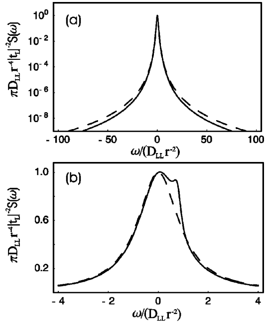
FIG. 1. In (a), we plot the spectrum (full line) in a log scale for \gamma_{nL} = 10 and \Delta_{nL} = 1 . In (b), we plot the spectrum in a linear scale for \gamma_{nL} = 0.2 and \Delta_{nL} = 0.8 . All rates are in units of D_{LL}/r^2 . We also plot in the same figures the Lorentzian spectrum for the laser mode alone (dotted line) that one would obtain if the coloring were negligible.
