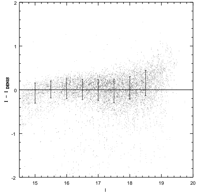
Fig. 6. Comparison of the EIS I-band magnitudes with those measured by DENIS for the two strips that overlap patch C ( top ) and patch D ( bottom ). Also shown are the mean and the rms in 0.5 mag bins.
