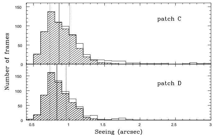
Fig. 1. The seeing distribution for the patches C and D obtained from all observed tiles (empty bars) and those actually accepted for the survey (shaded bars).
