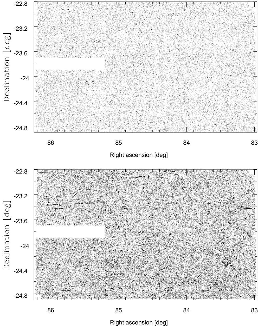
Fig. 7. The projected distribution of stars ( upper panel , I \leq 21.5 ) and galaxies ( lower panel , I \leq 22.5 ) from patch C.
