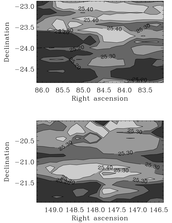
Fig. 4. Two-dimensional distribution of the limiting isophote as defined in the text estimated from the accepted even frames for patches C and D.
