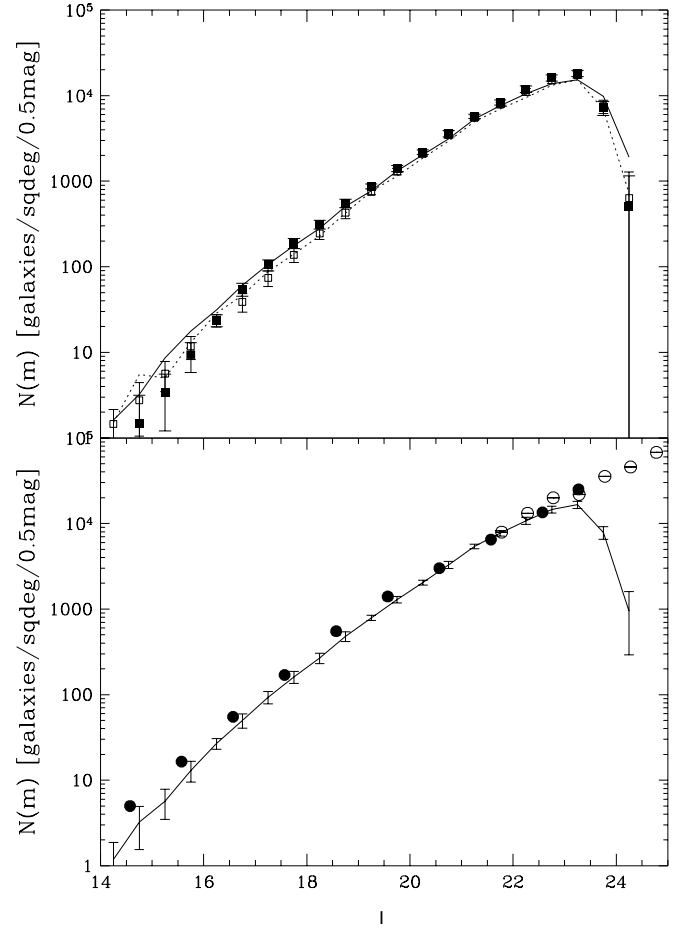
Fig. 10. Internal and external comparison of the EIS galaxy counts. Upper panel shows the counts for patch C (open squares) and patch D (filled squares), compared to the counts in patch A (solid line) and patch B (dotted line). Lower-panel shows the average counts for all EIS patches and the counts obtained by Postman et al. (1997) (filled circles) and HDF (open circles).
