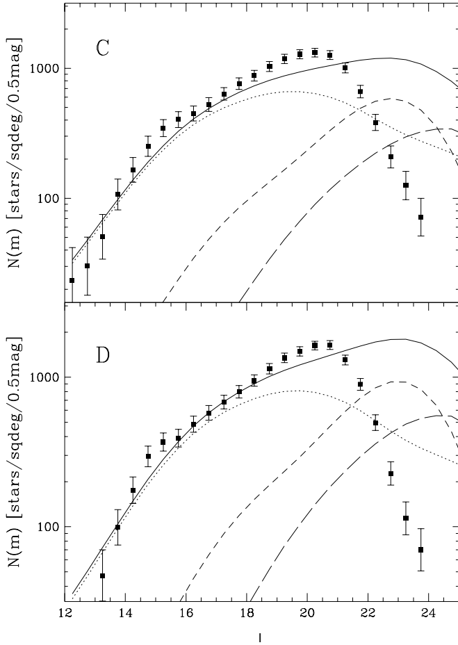
Fig. 9. The differential star counts versus the I-magnitude for patches C and D compared to model predictions (see text). The dotted line represents the disc, the dashed line the thick disc, the long-dashed line the halo, and the solid line the sum of the three.
