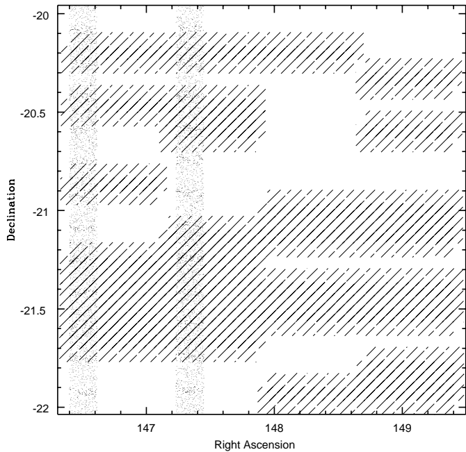
Fig. 5. Overlap of DENIS strips that cross the surveyed area of patches C ( top ) and D ( bottom ). The hatched area represents regions containing EIS frames observed under photometric conditions.
