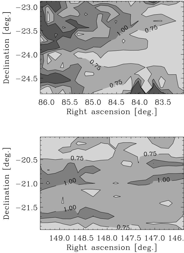
Fig. 3. Two-dimensional distribution of the seeing as measured for patches C (upper panel) and D (lower panel).
