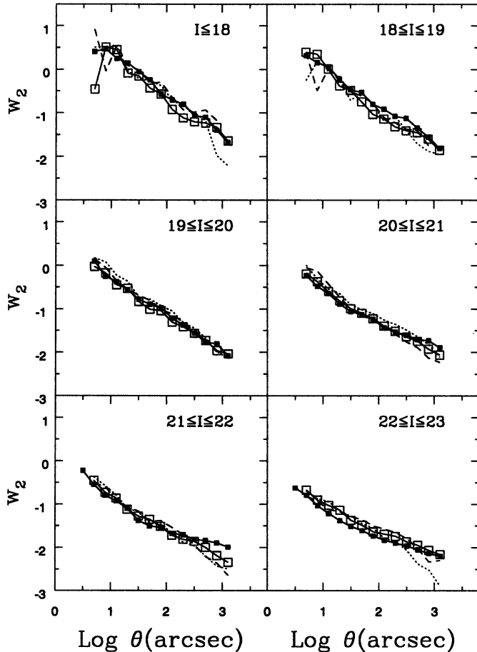
Fig. 11. Angular two-point correlation functions computed for patches C (open squares) and D (full squares). For comparison those obtained for patches A (dotted line) and B (dashed line) are also shown.
