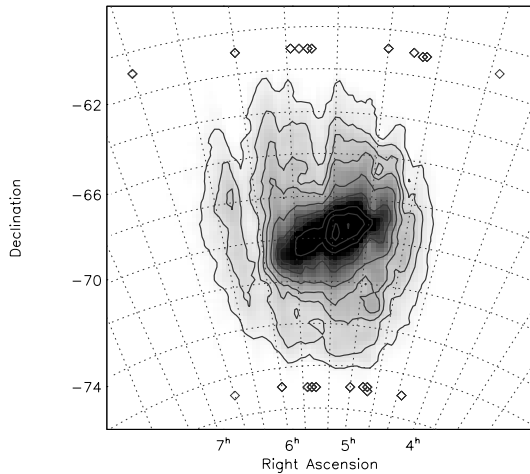
Fig. 4. Star count of the LMC – class C (Fig. 1); contours are at: 100, 150, 200, 250, 350, 500, 600, 800, 1000, 1200 per 0.04 \text{ deg}^2 .
