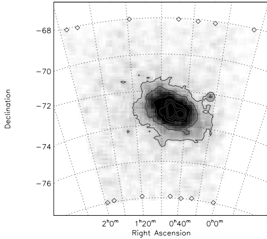
Fig. 6. Star count of the SMC – class B; contours are at: 2, 5, 10, 15, 20, 25, 50 per 0.04 \text{ deg}^2 .
