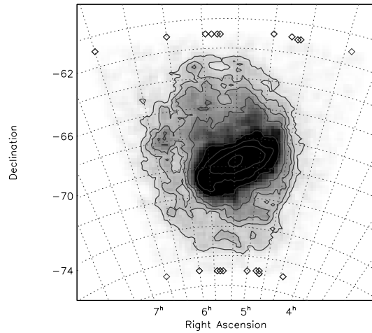
Fig. 3. Star count of the LMC – class B (Fig. 1); contours are at: 3, 5, 7, 10, 20, 30, 50, 100, 150 per 0.04 \text{ deg}^2 .
