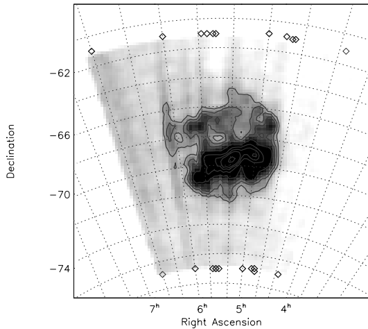
Fig. 2. Star count of the LMC – class A (Fig. 1); contours are at: 100, 125, 150, 200, 300, 400, 500, 800 per 0.04 \text{ deg}^2 .
