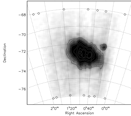
Fig. 7. Star count of the SMC – class C; contours are at: 50, 60, 75, 100, 125, 150, 200, 225 per 0.04 \text{ deg}^2 .
