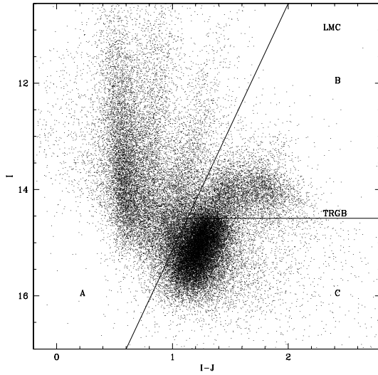
Fig. 1. Colour–Magnitude Diagram ( I - J, I ) of sources detected simultaneously in I, J and K_S towards the LMC ( -69 < \delta < -67 ). The horizontal line marking the position of the TRGB (Cioni et al. 2000a), and the slanted line at I < -4.64 \times (I - J) + 19.78 define the classes A, B, and C discussed in the text.
