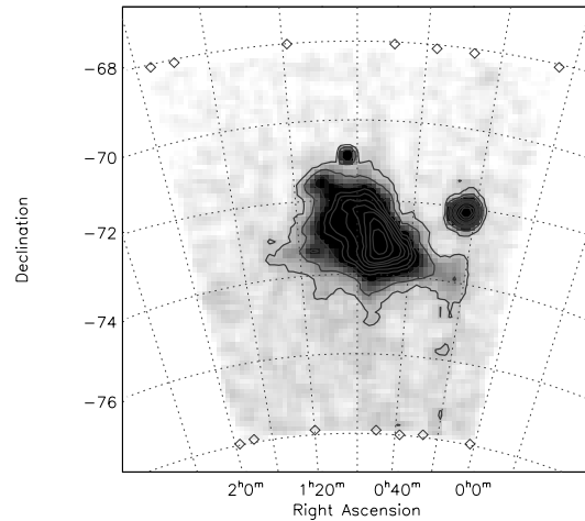
Fig. 5. Star count of the SMC – class A; contours are at: 20, 30, 45, 60, 75, 100, 125, 150, 200, 250 per 0.04 \text{ deg}^2 .
