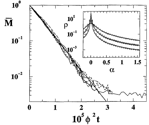
FIG 2 Decay of \bar{M} in the golden rule regime for kicking strengths K=13 , 17 , and 21 as a function of the rescaled time \phi^2 t . Perturbation strengths range from \phi=10^{-4} to 10^{-3} . Inset: Local spectral density of states for K=13 and perturbation strengths \phi=2.5 \times 10^{-4} , 5 \times 10^{-4} , 10^{-3} . The solid curves are Lorentzian fits, from which the decay rate \Gamma \approx 0.84 \phi^2 S^2 is extracted. The solid line in the main plot gives the decay \bar{M} \propto \exp(-\Gamma t) with this value of \Gamma .
