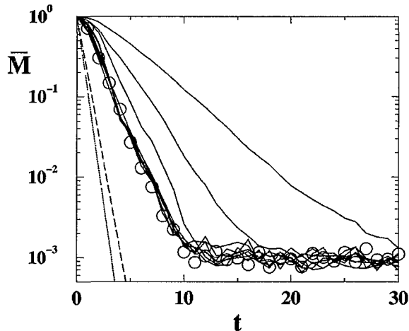
FIG 3 Decay of \bar{M} in the golden rule regime without rescaling of time, for K=13.1 , \phi=j \times 10^{-3} , ( j=1,1.5,2, \dots, 5 ) (solid curves) and K=21.1 , \phi=3 \times 10^{-3} (circles). Dashed and dotted lines show exponential decays with Lyapunov exponents \lambda=1.65 and 2.12 , corresponding to K=13.1 and 21.1 , respectively. The decay slope saturates at \phi \approx 2.5 \times 10^{-3} , when \Gamma reaches the bandwidth.
