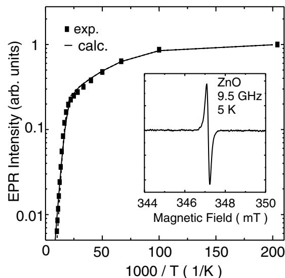
FIG. 1. The 9.5 GHz EPR signal of the shallow donors in ZnO (inset) and the dependence of its intensity on temperature. The solid line shows the result of the calculation according to Eq. (1).
