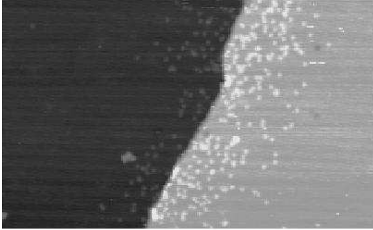
Fig. 1. 662 \times 404 \text{ \AA}^2 STM image of a monatomic height step on a Cu(001) surface taken 38 minutes after the deposition of 0.03 ML of indium at room temperature. Embedded indium atoms show up as bright dots with a height of 0.4 \text{ \AA} . The image shows a high density of embedded indium atoms near the step. ( V_t = -1.158 \text{ V} , I_t = 0.1 \text{ nA} )
