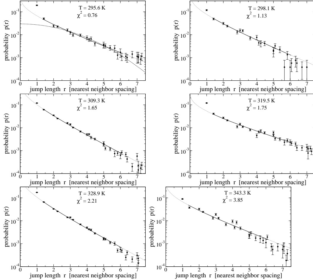
Fig. 6. Radial jump length distribution for embedded indium atoms measured for six different temperatures. The data points have been fitted with the modified Bessel function of order zero that is expected for the vacancy-mediated diffusion mechanism [14,15]. The fits were made to the data points for jump lengths from \sqrt{2} to 6, as indicated with the solid part of the curve in each panel. The normalized goodness of fit \chi^2 for this range is indicated. The dashed curve in the upper left panel is the best-fit Gaussian curve for the same data range.
