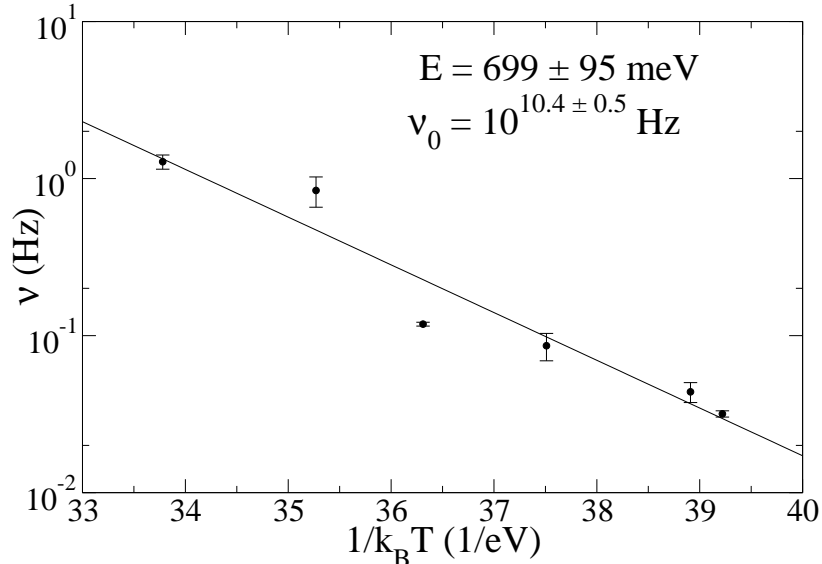
Fig. 8. Arrhenius plot of the rate of long jumps of the embedded indium atoms. The activation energy and attempt frequency are shown in the graph (see also fig. 11)
