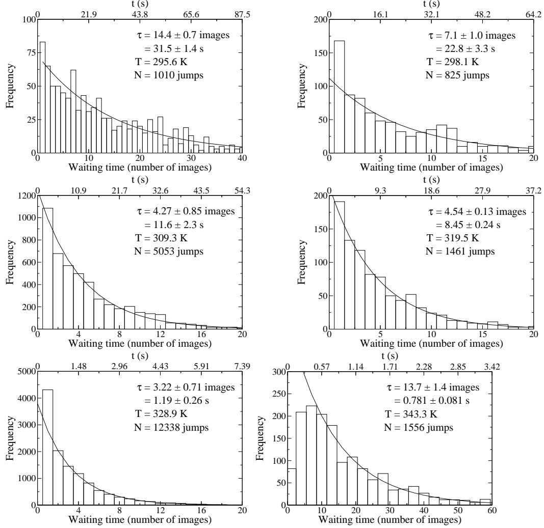
Fig. 7. Waiting time distributions measured for six different temperatures. All fits are pure exponentials. The time constant \tau is shown in the graph for each of the distributions. Too high or too low count rates at short waiting times are an artifact of the automated analysis scheme of the images [30,31] and are ignored in the fits.
