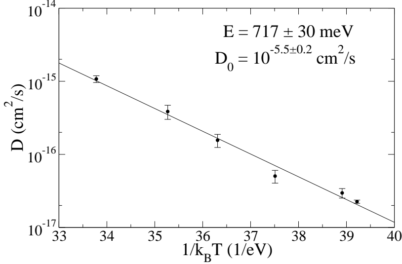
Fig. 11. Arrhenius plot of the diffusion coefficient D of embedded indium atoms. The coefficient D was calculated at each temperature by multiplying the rate of long jumps (figure 8) with the mean-square jump length (table 1).
