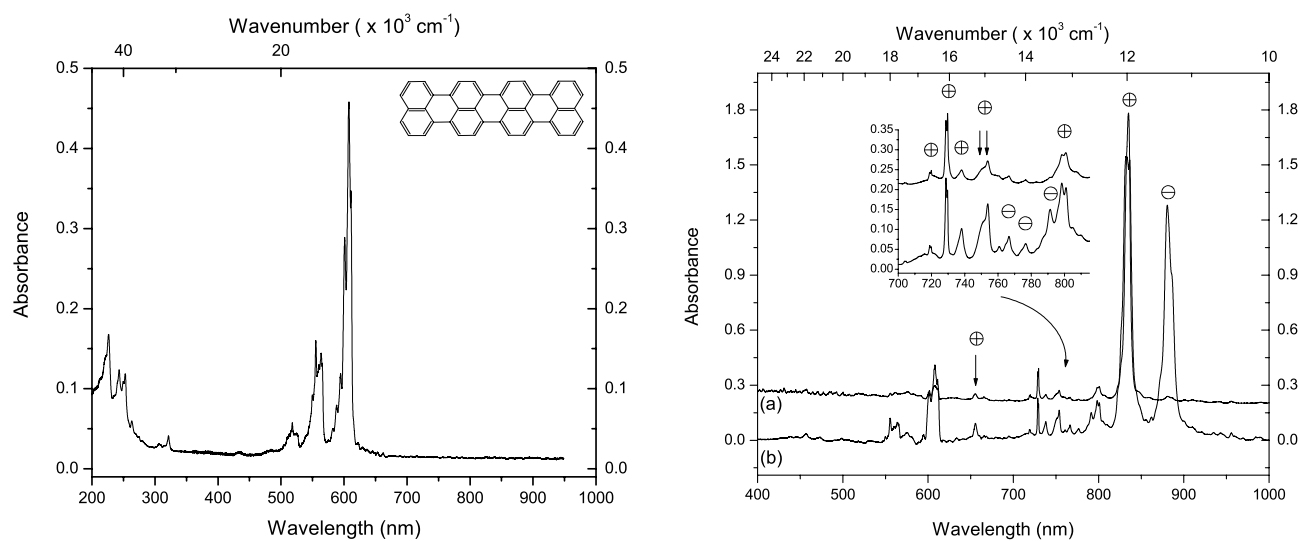
Fig. 7. Comparison of the spectral features associated with neutral (left panel) and VUV-irradiated (right panel) quaterylene (Qt) isolated in neon (Ne) and in Ne/ NO_2 matrices. a ) is the spectrum of the photolysis products in a neon/ NO_2 matrix; b ) is the spectrum of the photolysis products including, Qt^+ and Qt^- , in a neon matrix. Band peak positions, intensities and FWHM are given in Table 6.
