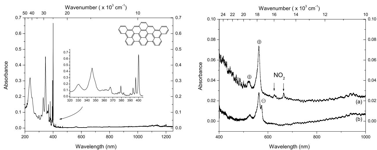
Fig. 8. Comparison of the spectral features associated with neutral (left panel) and VUV-irradiated (right panel) hexabenzoperopyrene (Hp) isolated in neon (Ne) and in Ne/ NO_2 matrices. a ) is the spectrum of the photolysis products in a neon/ NO_2 matrix; b ) is the spectrum of the photolysis products, including Hp^+ and Hp^- , in a neon matrix. Band peak positions, intensities and FWHM are reported in Table 7.
