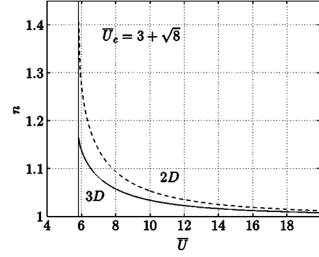
FIG. 10. Total density n at T=0 as a function of interaction strength \bar{U}=U/zt for the first Mott lobe in two (dashed line) and three dimensions (solid line) when including fluctuations. The density approaches a finite value different from 1, when approaching U_c .
