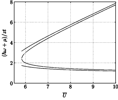
FIG. 8. Dispersion relations \hbar\omega + \mu as a function of U/zt for \mathbf{k}=\mathbf{0} for zero and nonzero temperatures. The inner lobe corresponds to zero temperature. The outer lobe corresponds to a temperature of zt\beta=3 . Here we have only taken into account the first three terms in the right-hand side of Eq. (18), i.e., in the sum we only include the terms with \alpha=0 and \alpha=1 .
