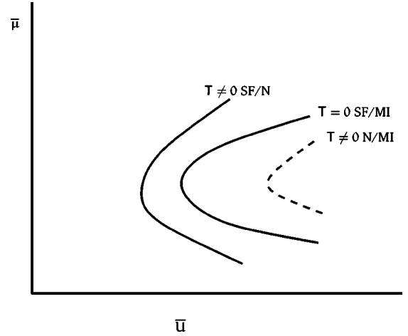
FIG. 2. Qualitative phase diagram in terms of the chemical potential \bar{\mu}=\mu/zt and the dimensionless coupling constant \bar{U}=U/zt . The solid lines indicate real phase transitions between superfluid, normal, and Mott insulating phases. the dashed line corresponds to a crossover between a normal and a Mott insulating phase.
