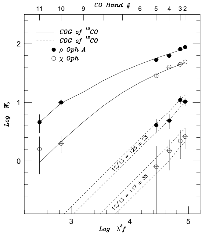
FIG. 5.—Curves of growth for the A - X system of bands in 12 CO (solid lines) and 13 CO (dashed lines) toward \rho Oph A (filled circles) and \chi Oph (open circles). The numbers along the top give v' for the band. The resulting 12 CO/ 13 CO ratios are also indicated.
