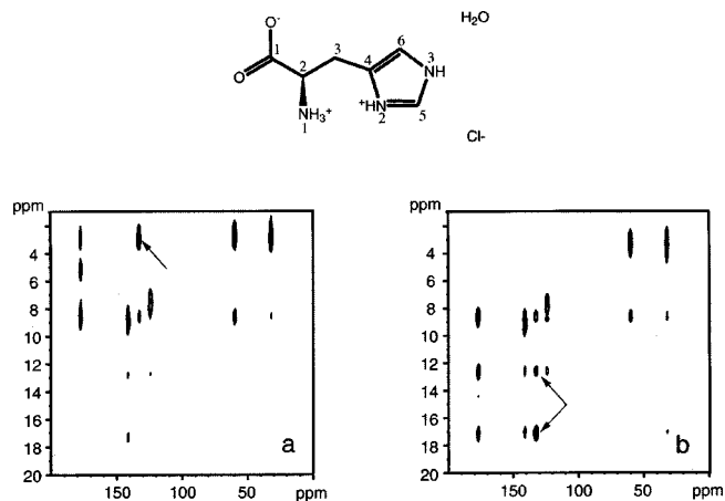
FIG. 8. The structure of [ 13 C, 15 N] histidine.HCl.H 2 O and 2D heteronuclear correlation spectra obtained from the experiment shown in Fig. 1(b) with \tau = 0.8 ms. The spectrum in (a) results from an experiment in which the polarization transfer efficiency between the protons of C β and 4- 13 C was maximized. An arrow points to the corresponding cross peak. The cross peak intensities corresponding to 2- 15 NH and 3- 15 NH with 4- 13 C are below the contour limits. In 2D LG-CP spectrum in (b) the proton carrier frequency was moved and the cross peaks between the 2- 15 NH and 3- 15 NH protons and 4- 13 C become stronger (indicated by arrows), whereas the polarization transfer with the protons of 13 CH 2 is significantly reduced.
