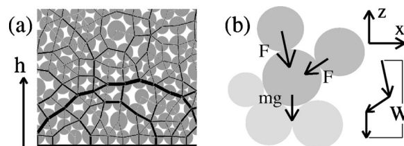
FIG. 1. (a) Detail of a typical packing in our simulations; the height h denotes the distance from the bottom. The force network is represented by the black lines whose thickness is proportional to the force magnitude. (b) Definition of interparticle forces F and weight W , for a frictionless particle with n_c=2 ; see Eq. (1).
