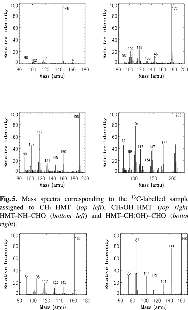
Fig. 6. Mass spectra corresponding to the ^{13}C (left panel) and ^{15}N (right panel) labelled peaks attributed to HMT-OH.
