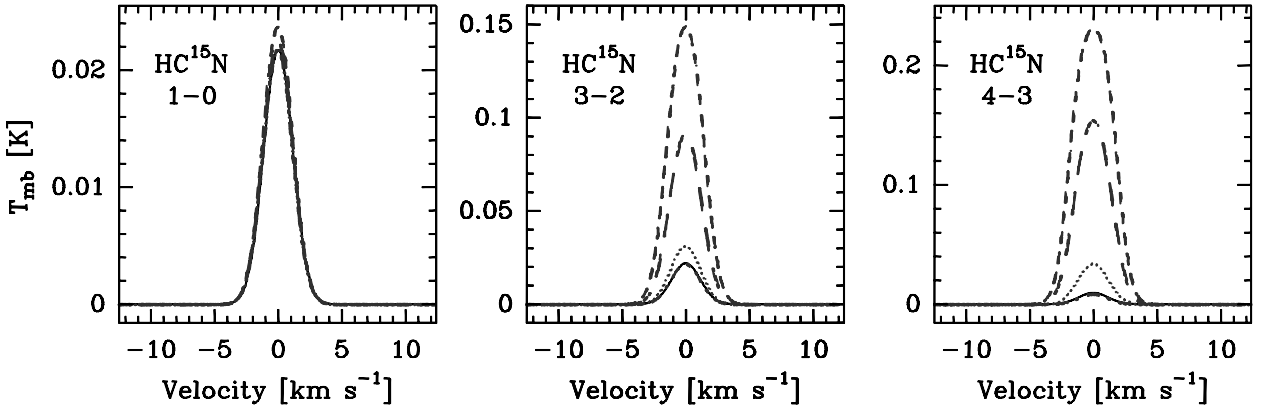
Fig. 9. \text{HC}^{15}\text{N} line profiles calculated for different UV fields. Solid line: G_{0,\text{in}} = 0 . Dashed line (small): G_{0,\text{in}} = 10 . Dashed line (big): G_{0,\text{in}} = 100 . Dotted line: G_{0,\text{in}} = 10^3 . Dash-dotted line: G_{0,\text{in}} = 10^5 . The \text{HC}^{15}\text{N} 1–0 transition has a frequency of 86 GHz (convolved to a 63'' NRAO beam), the 3–2 transition has a frequency of 258 GHz (convolved to a 20'' JCMT beam) and the 4–3 transition has a frequency of 344 GHz (convolved to a 14'' JCMT beam). The size of the source is approximately 30'' (29 000 AU).
