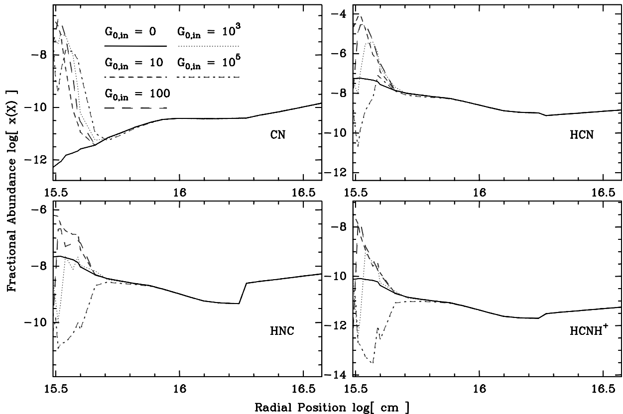
Fig. 6. Depth-dependent fractional abundances of CN, HCN, HNC and HCNH + for different UV fluxes.
