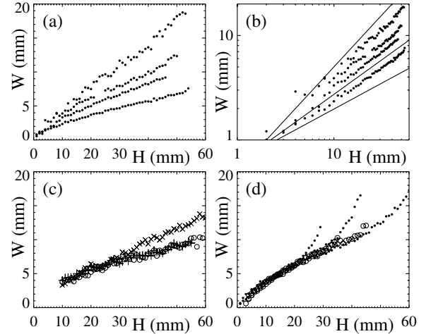
FIG. 5. Width of the shear zones versus H . (a) Linear and (b) log-log plots of W for spherical glass beads of increasing sizes for R_s = 95 mm (mixture I-IV). The width grows with particle size. The straight lines in (b) have slopes 1/2 , 2/3 , and 1 , showing that W grows faster than \sqrt{H} but slower than H . (c) Irregular particle shapes diminish W substantially, as can be seen by comparing the widths for the plastic flakes (V/pluses), aluminum oxide beads (VI/open circles), and coarse sand (VII/crosses) to those of the glass beads shown in panel (a). (d) W for mixture III and R_s = 95, 85, and 75 mm (Couette geometry; open symbols) and R_s = 95, 65, and 45 mm (disk geometry; closed symbols). The strong upward deviations observed in the disk geometry coincide with the symmetry breaking of the velocity profiles (see text). Apart from this, the setup geometry does not affect W .
