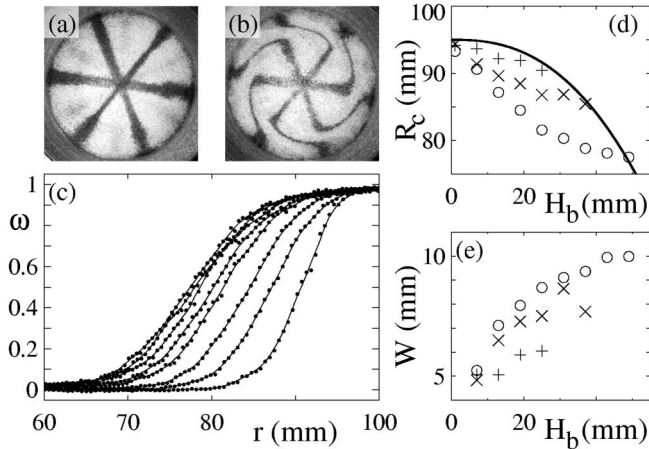
FIG. 6. Measurements of \omega(r) inside the material for the disk geometry and R_s = 95 mm. (a) Initial pattern at H_b = 31 mm. (b) The same pattern after adding material up to H = 49 mm, rotating, and removing the upper layers. (c) Velocity profiles for H = 49 mm, and H_b = 7, 13, 19, \dots, 49 mm (from right to left). (d) R_c(H_b) for H = 25 mm (plusses), H = 37 mm (crosses), and H = 49 mm (circles) compared to R_c(H) given by Eq. (2) (curve). (e) Corresponding W(H_b) .
