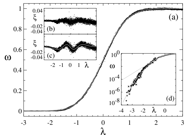
FIG. 3. (a) Collapse of all 35 bulk profiles obtained for H = 4, 5, 6, \dots, 38 mm (mixture I, R_s = 85 mm, as in Fig. 2) when plotted as function of the dimensionless coordinate \lambda := (r - R_c)/W . The gray curve is an error function. (b) Differences \xi between bulk profiles and fits to Eq. (1). (c) Differences \xi between bulk profiles and fits to 1/2 + 1/2 \tanh(l\lambda) , where l \approx 1.20274 compensates for the difference in scale between error function and hyperbolic tangent. The gray curve shows [\operatorname{erf}(\lambda) - \tanh(l\lambda)]/2 . (d) Left tail of the velocity profile in log-linear scale, compared to the best fit to either a hyperbolic tangent and error function (gray curves). Dots, crosses, and plusses are obtained for time lags 0.3, 3, and 30 s, respectively.
