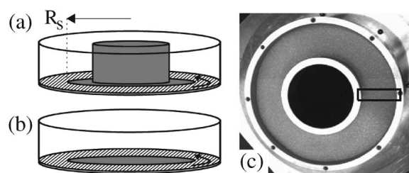
FIG. 1. (a) Schematic side-view of our split-bottomed Couette cell, showing the stationary bottom disk and inner cylinder (both gray), and the rotating bottom ring (striped) and outer cylinder. A thin layer of felt between the rings assures smooth rotation. The inner and outer cylinder radii are fixed at 65 and 105 mm, respectively, while R_s can be varied. (b) Setup in disk geometry. (c) Top view of the filled set up in the Couette geometry, where the rectangle indicates the area recorded by the video camera.
