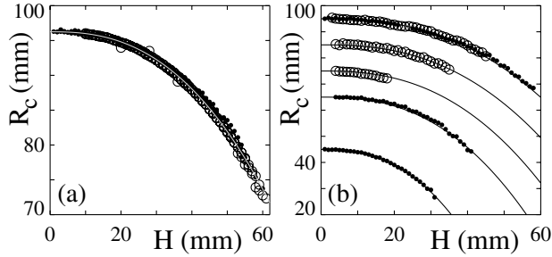
FIG. 4. Shear zone positions R_c versus height, where H is restricted to the universal regime detected by a \chi^2 test. (a) Comparison between R_c(H) for glass beads I-IV (closed symbols), nonspherical particles V-VII (open symbols) and Eq. (2) (curve). For all runs, R_s is 95 mm. (b) R_c(H) for mixture III and R_s = 95, 85, and 75 mm in the Couette geometry (open symbols) and R_s = 95, 65, and 45 mm in the disk geometry (closed symbols), compared to Eq. (2) (curves).
