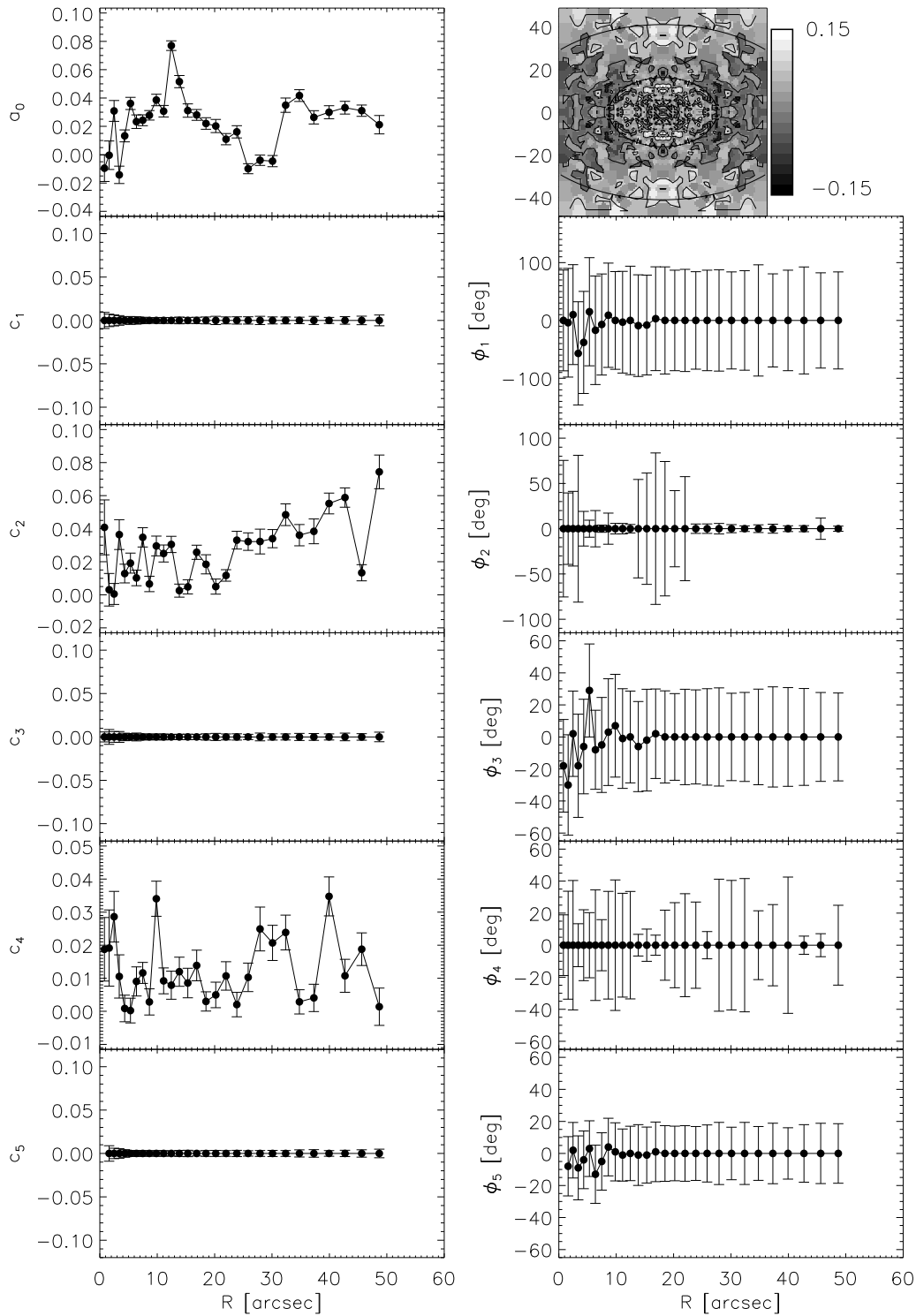
Figure 5 — Kinematic expansion of the h_4 map of the model axisymmetric galaxy. Panels on the left column show amplitude coefficients of the kinematic expansion (from top to bottom): a_0, c_1, c_2, c_3, c_4 and c_5 . The h_4 map is presented in the upper right panel, while the other panels show the same phase angles as in Fig 2, but for the h_4 map.
