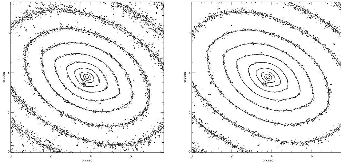
Figure B.2 — Contour maps of WFC2 F450W (left) and F555W (right) images of NGC 4128. The images show the inner 7''.5 . Superposed on the two images are the contours of the MGE surface brightness, convolved with the WFC2 PSFs for the corresponding filters. The transient was excluded from the fit, but it is shown in the images for illustration.
