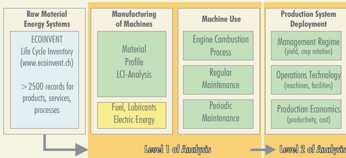
Fig. 1 Components of the analytical framework. The production system is the highest hierarchical level consisting of components of the next lower level, the machine. There are three types of data: (1) own original data and meta-data [green boxes], (2) standard life cycle inventory data Ecoinvent [blue box], and (3) data that were not available [yellow box].
