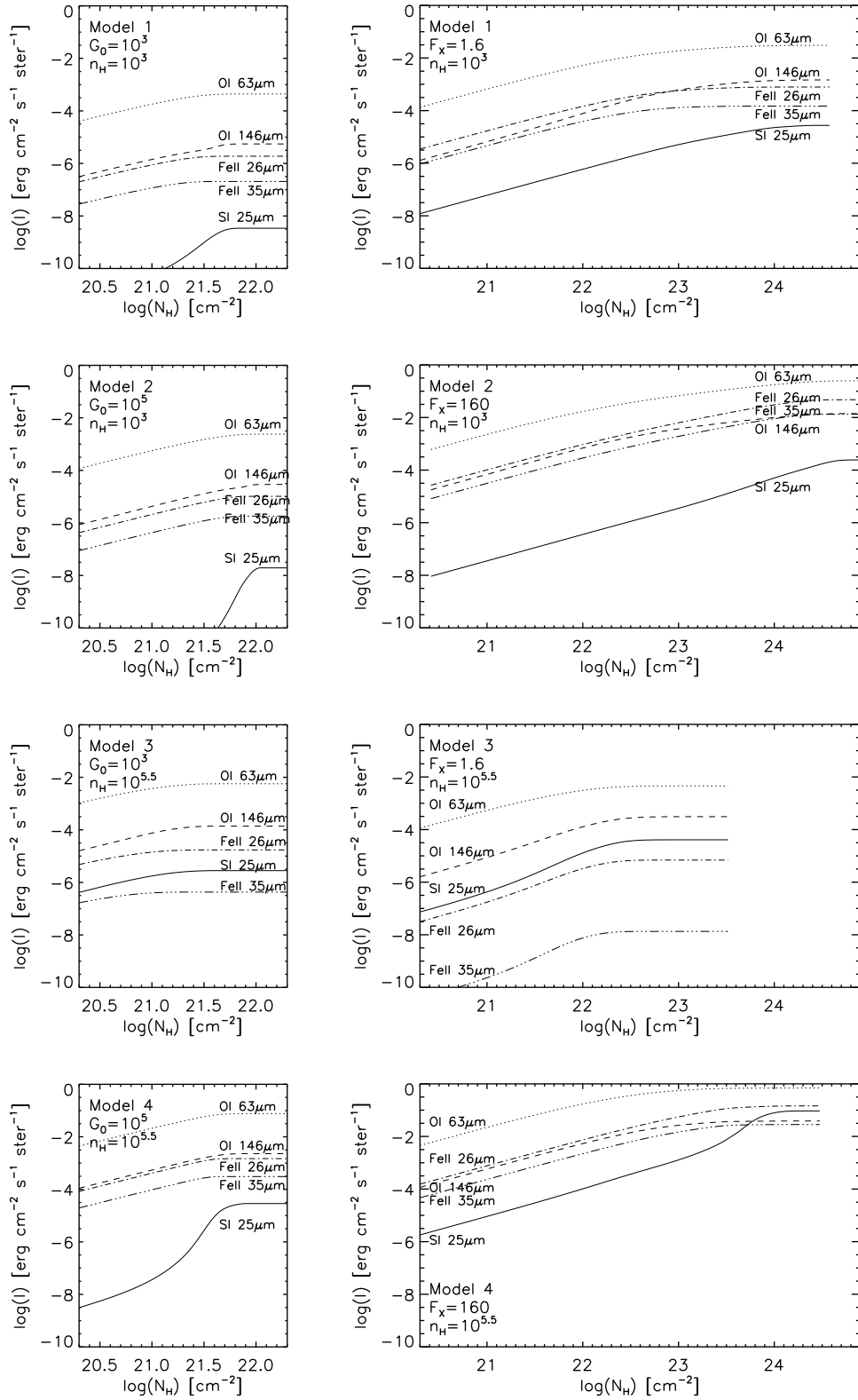
Figure 6.10: Cumulative line intensities of [SI] 25.2 (solid), [OI] 63.2 (dotted), 145.6 (dashed), [FeII] 26.0 (dot-dashed) and 35.4 μm (dotted-dashed), for PDR (left) and XDR (right) models.
