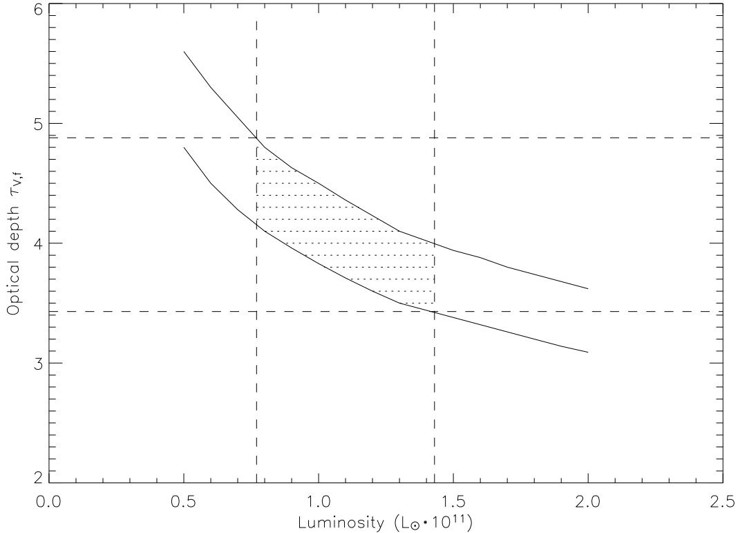
Figure 3.4: Resulting optical depth for different luminosities assuming either zero CO contamination (upper line) or an omnipresent maximum 12 per cent contamination (lower line). The shaded area shows the possible solutions.
