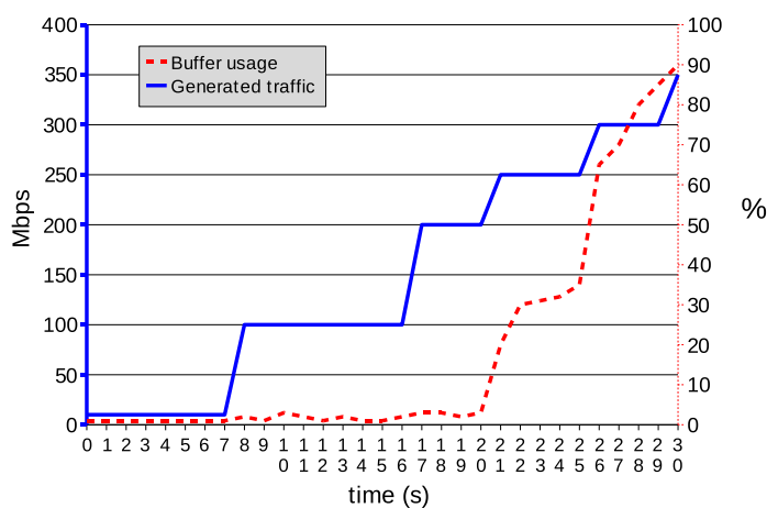
Figure 7.8: The workload measured on Node_1 .
