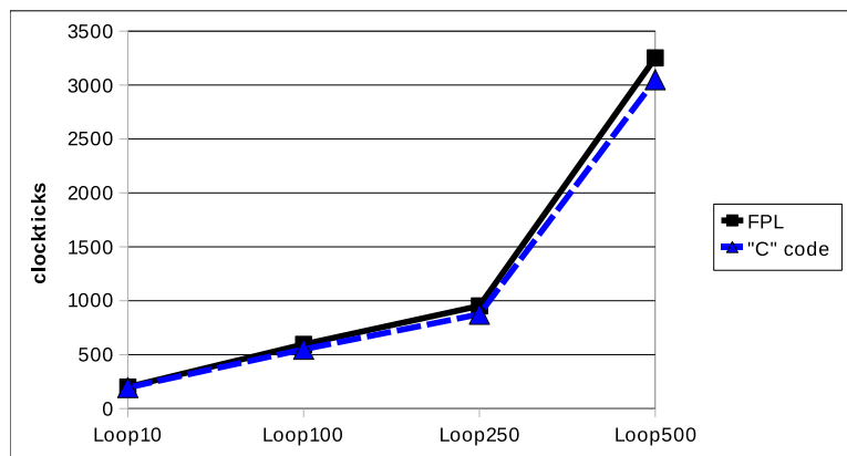
Figure 3.6: FPL versus "C" code.
