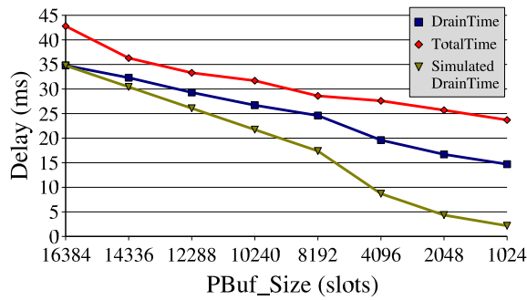
Figure 7.4: Tasks moving benchmark.
