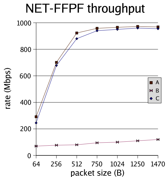
Figure 5.9: Benchmark result.
