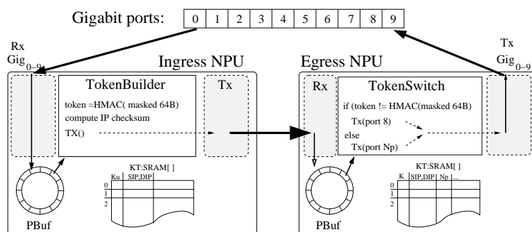
Figure 8.6: Token Based Switch using a dual IXDP2850.
