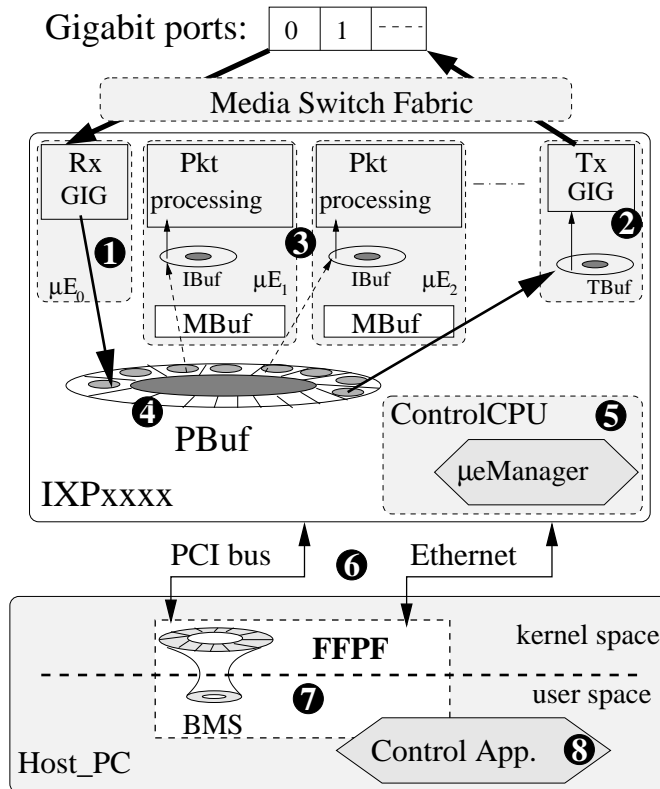
Figure 4.6: NIC-FIX architecture.
