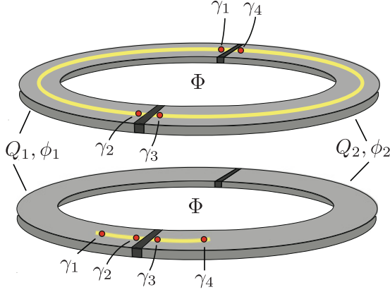
FIG. 1. (Color online) Geometry of a DC SQUID, consisting of a superconducting ring (gray) interrupted by two tunnel junctions (black) and threaded by a magnetic flux \Phi . A semiconductor nanowire (yellow) contains Majorana fermions at the end points (red dots). The two panels distinguish the cases that Majorana fermions are present at both junctions (top), or only at a single junction (bottom). The 4\pi -periodic Josephson effect is stable against quantum phase slips in the first case, but not in the second case.
