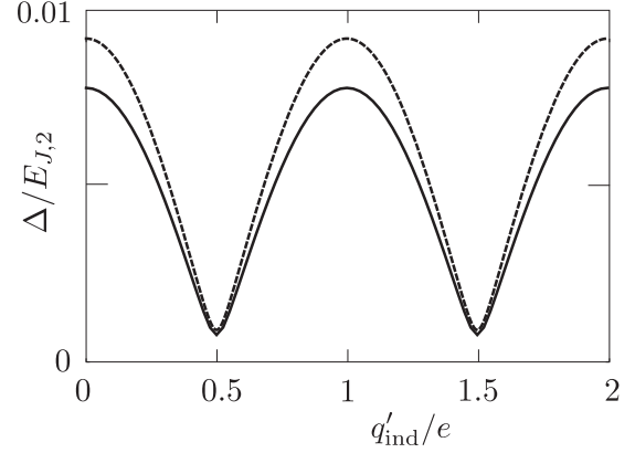
FIG. 4. Tunnel splitting at \varphi_0 = \pi as a function of the induced charge. The dashed curve corresponds to Eq. (15), the solid curve to numerical calculations for the full Hamiltonian, for E_{J,2} = 5E_C = 25E_{M,1} (with E_{M,2} = 0 = E_{J,1} ).
