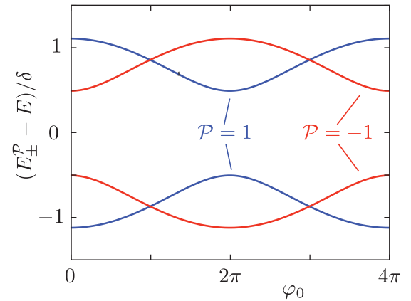
FIG. 2. (Color online) Spectrum of the DC SQUID in the top panel of Fig. 1, containing Majorana fermions at both Josephson junctions. The curves are the result (13), in the limit that the charging energy dominates over the Josephson energy. The parameters chosen are E_{M,1} = E_{M,2} = \delta . The level crossing is between states of different fermion parity \mathcal{P} , and therefore there can be no tunnel splitting due to the Coulomb interaction (which conserves \mathcal{P} ).
