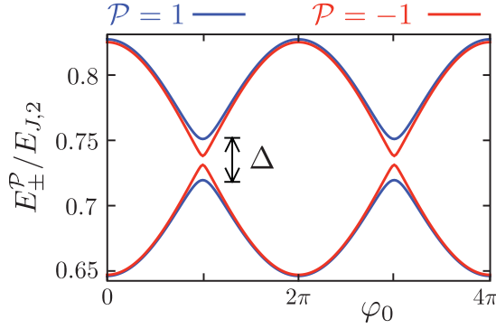
FIG. 3. (Color online) Spectrum of the DC SQUID in the bottom panel of Fig. 1, containing Majorana fermions at only one of the two Josephson junctions. The curves are a numerical calculation for the full Hamiltonian, in the regime that the Josephson energy of the trivial junction is the largest energy scale. The parameters chosen are E_{J,2} = 4E_C = 10E_{M,1} , E_{M,2} = 0 = E_{J,1} , and q_{\text{ind}} = 0 . In contrast to Fig. 2, a tunnel splitting \Delta appears because the level crossing is between states of the same fermion parity.
