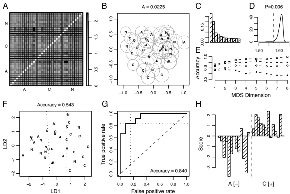
Figure 6. Distance-based analysis of normalized probability distributions of combined Rrs and Xrs in a 3+3 dimensional embedding. (A) Distance matrix for all subject-wise comparisons of signals by Wasserstein distances. (B) Two-dimensional MDS representation depicting the two major axes of variation. Each subject is represented by a point in this functional space (A: asthma, C: COPD, N: healthy controls), approximating the measured distances as close as possible. Misrepresentation error is indicated (by circles whose area is equal to stress-per-point), and the value of A (eq. (8)) given. (C) Relative size of eigenvalues of the scalar product matrix obtained from the distances, as a measure of explained variance. (D) Distribution of the MRPP statistic \delta . The value of \delta for the original groups is indicated (broken line). The fraction of permutations to the left of this is the significance probability (P-value) that the distances are not structured with respect to group membership. (E) Classification accuracies with respect to the number of MDS dimensions. Circles: full contrast, cross-validated ( \bullet ) and resubstitution accuracy ( \circ ). Squares: asthma/COPD contrast, cross-validated ( \blacksquare ) and resubstitution accuracy ( \square ). (F) Discriminant functions for full classification in a two-dimensional reconstruction. The decision boundaries are indicated (dotted lines). (G) Receiver-operator-characteristic for the discrimination of asthma (negatives) against COPD (positives) in the optimal five-dimensional reconstruction. Sensitivity (true positive rate, 0.83) and specificity ( 1 - \text{false positive rate} , 0.85) for the optimal threshold are indicated (broken lines), resulting in an accuracy of 0.84. (H) Corresponding discriminant scores for all subjects.
