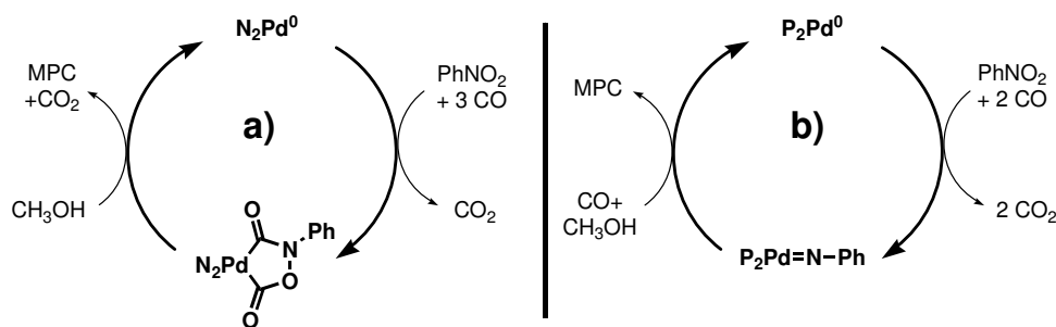
Scheme 6.2. Two simplified mechanistic proposals for the reductive carbonylation of nitrobenzene, catalyzed by a L_2Pd -catalyst wherein: a) L_2 is the N_2 -donor ligand 1,10-phenanthroline; b) L_2 is a P_2 -donor ligand such as bidentate diarylphosphanes.
