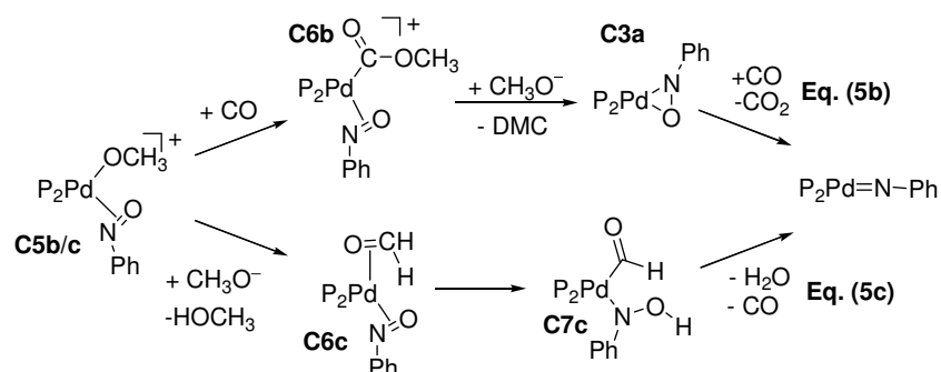
Scheme 3.5. Mechanistic proposals for nitrobenzene reduction to \text{P}_2\text{Pd}^{\text{II}}=\text{NPh} with either \text{CH}_3\text{OH}/\text{CO} as co-reductants (top, using only the -OH proton of methanol, eq. 5b) or with only \text{CH}_3\text{OH} as reductant (bottom, also using the -CH 3 protons of methanol, eq. 5c).
