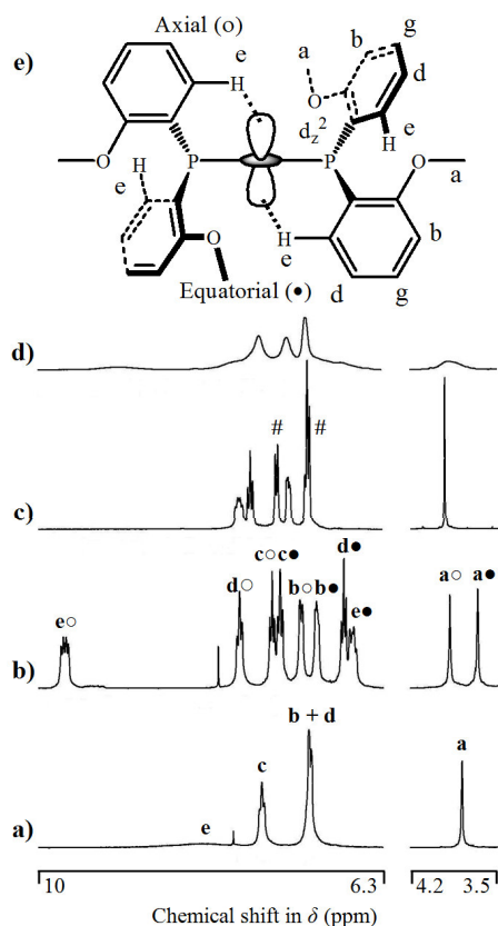
Figure 2.3. ^1\text{H-NMR} spectra of monochelate complexes in (\text{CD}_3)_2\text{CO} : a) M(\text{oMeO-L3X}^R)\text{A} at 23\text{ }^\circ\text{C} ; b) M(\text{oMeO-L3X}^R)\text{A} at -60\text{ }^\circ\text{C} ; c) M(\text{oMeO-L3X}^R)\text{T} at 23\text{ }^\circ\text{C} ; d) M(\text{oMeO-L3X}^R)\text{T} at -60\text{ }^\circ\text{C} ; e) schematic view of the interactions and labeling of the H atoms. An ‘•’ indicates that the resonance belongs to an equatorially aligned ring, ‘o’ indicates that the resonance belongs to an axially aligned ring, and ‘#’ indicates a resonance from a tosylate anion.
