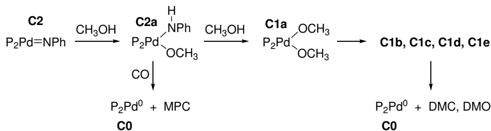
Scheme 5.9. Proposed mechanism for the formation of the ‘second’ equivalent of DMC and DMO (and aniline) in competition with MPC production.
