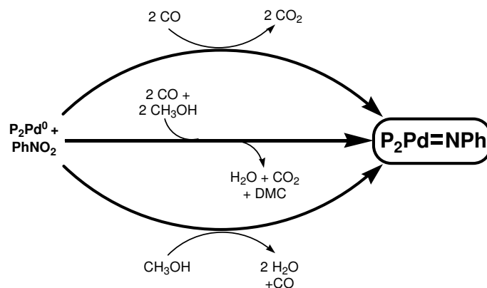
Scheme 3.6. Three competing pathways for the reduction of nitrobenzene to a \text{Pd}^{\text{II}} -imido intermediate, using two CO (top), one CO and the acidic protons of two methanol (centre) or all H-atoms of one methanol (bottom) as de-oxygenating agent.
