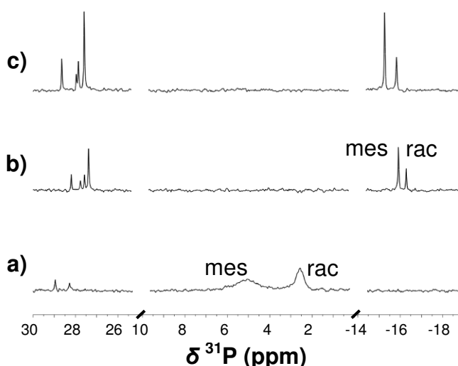
Figure 4.20. ^{31}\text{P}\{^1\text{H}\} -NMR spectra of reaction mixtures for the in situ formation of [(\text{bpap})\text{Pd}=\text{NMes}] in d^8 -toluene, from [\text{Pd}(\text{bpap})(\text{dba})] and mesitylene azide: (a) pure [\text{Pd}(\text{bpap})(\text{dba})] ; (b) after mesitylene azide addition and heated at 100 °C; (c) after cooling to room temperature.
