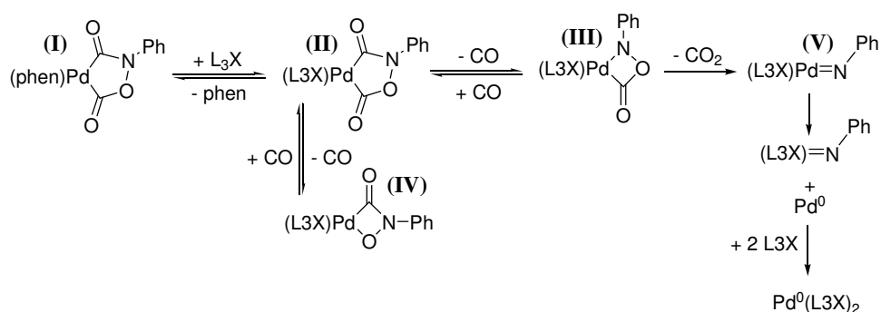
Scheme 4.4. Proposed reaction sequence of the ligand exchange between 'phen-palladacycle' ( I ) and the diposphane ligand L3X, followed by decomposition of the 'L3X-palladacycle' ( II ).
