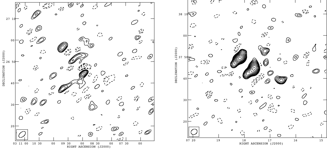
(a) MACSJ0308+26. The 1\text{-}\sigma map noise is 141\ \mu\text{Jy beam}^{-1} . Contour levels start at \pm 280\ \mu\text{Jy beam}^{-1} ; thereafter contours are spaced by a factor of \sqrt{2} .
