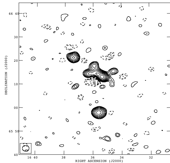
(d) A2218. The 1\text{-}\sigma map noise is 88 \mu\text{Jy beam}^{-1} . Contour levels start at \pm 180 \mu\text{Jy beam}^{-1} ; thereafter contours are spaced by a factor of \sqrt{2} .
