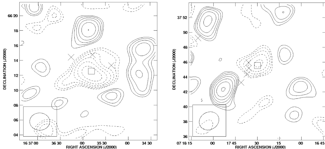
(a) A2218. The 1\text{-}\sigma map noise is 88 \mu\text{Jy beam}^{-1} . Contour levels start at \pm 180 \mu\text{Jy beam}^{-1} ; thereafter contours are spaced by a factor of \sqrt{2} .
