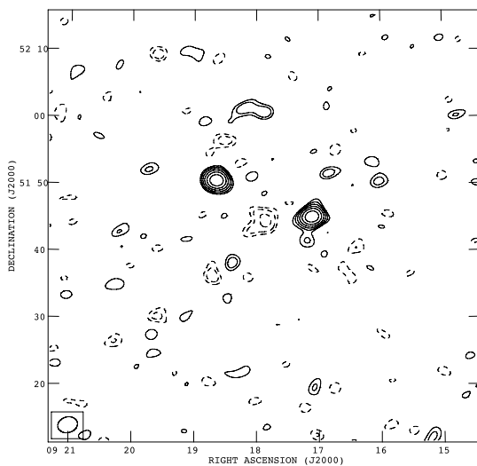
(c) A773. The 1\text{-}\sigma map noise is 157 \mu\text{Jy beam}^{-1} . Contour levels start at \pm 310 \mu\text{Jy beam}^{-1} ; thereafter contours are spaced by a factor of \sqrt{2} .
