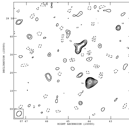
(c) MACSJ0744+39. The 1\text{-}\sigma map noise is 317\ \mu\text{Jy beam}^{-1} . Contour levels start at \pm 630\ \mu\text{Jy beam}^{-1} ; thereafter contours are spaced by a factor of \sqrt{2} .
