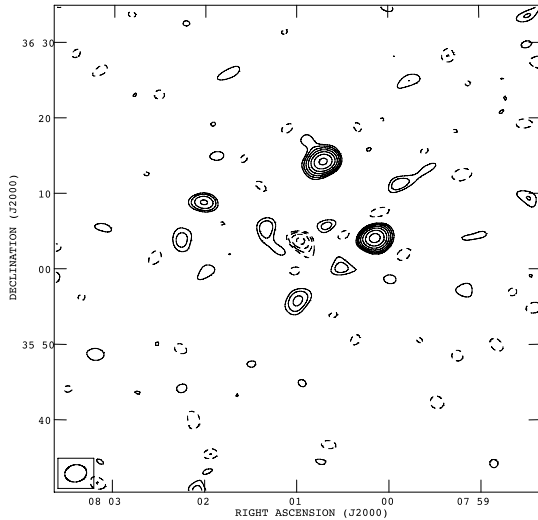
(a) A611. The 1\text{-}\sigma map noise is 139 \mu\text{Jy beam}^{-1} . Contour levels start at \pm 280 \mu\text{Jy beam}^{-1} ; thereafter contours are spaced by a factor of \sqrt{2} .
