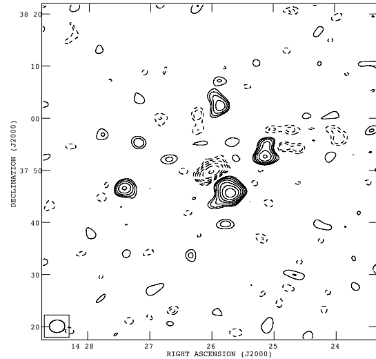
(b) A1914. The 1\text{-}\sigma map noise is 144 \mu\text{Jy beam}^{-1} . Contour levels start at \pm 290 \mu\text{Jy beam}^{-1} ; thereafter contours are spaced by a factor of \sqrt{2} .
