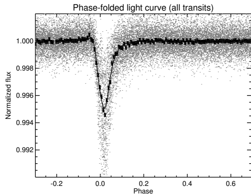
Fig. 1. The normalized light curve of KIC 1255b, phase-folded using a period of P = 15.6854 h. A binned light curve (solid squares, with error bars) and the best-fit model (solid line) are overlotted.
