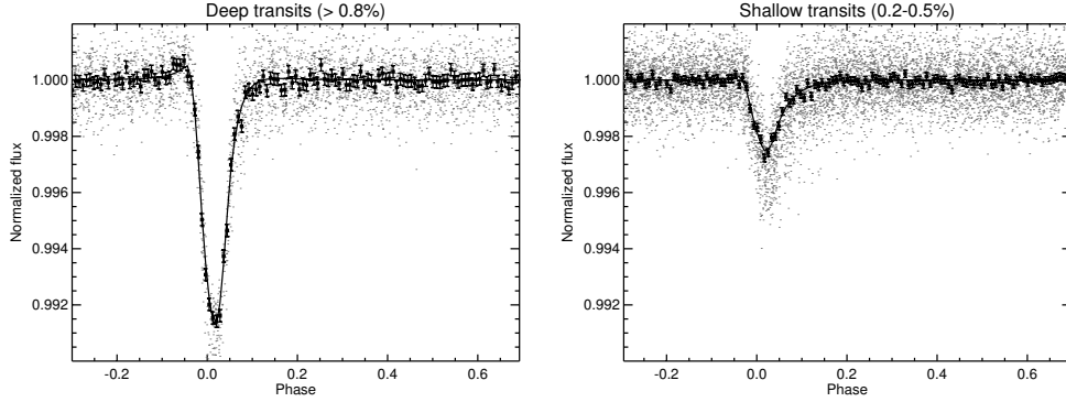
Fig. 3. Light curves of KIC 1255b, obtained by dividing the events into two groups based on their transit depths and binning the photometry by 0.008 in phase. The left panel shows the average light curve of the deep events (deeper than 0.8%), and the right panel shows the average light curve of the shallow events (depths between 0.2% and 0.5%). The best-fit models for the two light curves are shown as a solid line.
