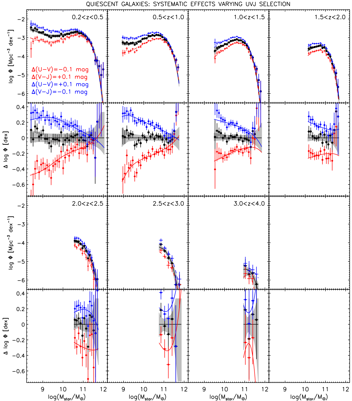
Figure 19. As in Figure 15 but for quiescent galaxies with two different definitions of star-forming and quiescent galaxies. Varying the selection has a much stronger effect on the derived mass functions for high masses than low masses because high-mass galaxies are the most quiescent.
