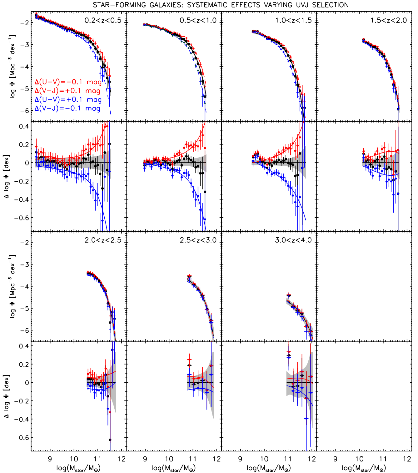
Figure 20. As in Figure 15 but for star-forming galaxies with two different definitions of star-forming and quiescent galaxies. The effect of different definitions of quiescent on the star-forming population is opposite to that on quiescent galaxies. Low-mass galaxies are not affected because they have the highest SSFRs, whereas the most massive star-forming galaxies have much lower SSFRs.
