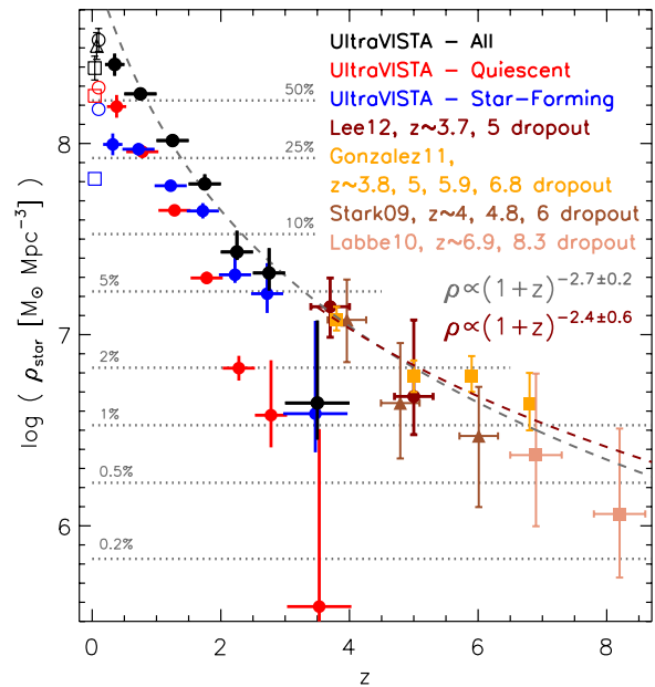
Figure 13. Evolution of the stellar mass density in the universe between z = 0-8.5 . The SMDs determined from UV-selected samples are shown at z > 3.5 . Below z < 3.5 , the K_s -selected SMDs from UltraVISTA are shown for the total (black), star-forming (blue), and quiescent (red) populations. The z \sim 0 data from Cole et al. (2001; triangles), Bell et al. (2003; circles), and Baldry et al. (2012; squares) are also shown. The SMD in star-forming galaxies from the K_s -selected and UV-selected samples agrees to within 1\sigma , suggesting that UV-selected samples account for most of the SMD at z > 3.5 . The dashed gray curve shows a simultaneous fit to the total SMD from UltraVISTA at z > 1.5 and the UV-selected samples and the dashed maroon curve shows a fit to just the UV-selected samples, both of which agree well.
