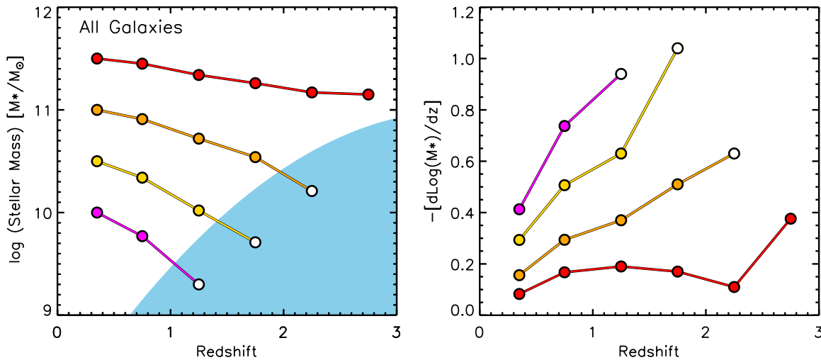
Figure 14. Left panel: average stellar mass of galaxies chosen at a fixed cumulative number density from the Schechter function fits. The cumulative number densities are chosen so that they correspond to galaxies with \log(M_{\star}/M_{\odot}) = 11.5, 11.0, 10.5, and 10.0 in the lowest redshift SMF. The shaded blue region represent the region that requires extrapolating the Schechter function beyond the depth of the data. Right panel: derivatives of the growth in stellar mass as a function of redshift. The derivatives separate into a sequence showing that the rate mass growth is always larger for lower mass galaxies at z < 2 .
