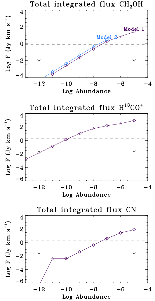
Fig. 12. Model results for the integrated fluxes found for CH 3 OH, H 13 CO + and CN in the empirical models. The dashed line indicates the upper limit of the integrated intensity, assuming the molecule is cospatial with the H 2 CO (CH 3 OH) or CO (H 13 CO + and CN). Abundances were calculated with respect to the CO abundance, but in these plots are multiplied with 10 -4 to translate the abundance w.r.t. CO to H 2 .
