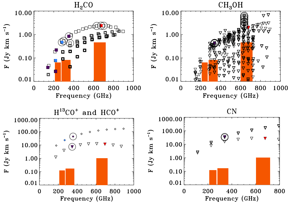
Fig. 13. Model predictions for the integrated fluxes for \text{H}_2\text{CO} (both ortho and para lines, assuming an ortho/para ratio of 3), and upper limits for A- \text{CH}_3\text{OH} , \text{H}^{13}\text{CO}^+ , \text{HCO}^+ (triangles and diamonds, respectively), and CN based on our best-fit models for detections and upper limits. The boxes show the 3\sigma upper limit of the ALMA sensitivity for Band 6 (230 GHz), Band 7 (345 GHz), and Band 9 (690 GHz), integrated over the line profile for one hour integration in the full array. The targeted lines in observations are indicated in red (this study), blue (Öberg et al. 2010, 2011), and purple (Thi et al. 2004). The lines that have the best potential for observation compared with the ALMA sensitivity are encircled.
