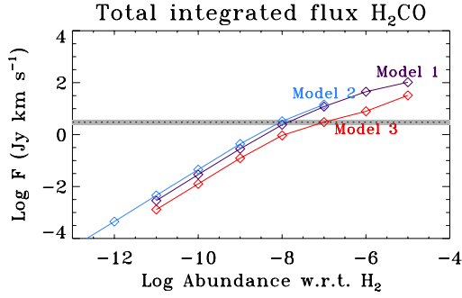
Fig. 7. Results of H 2 CO abundance models: total flux integrated over the emission rectangle of the observations for different abundances for model 1 (purple), model 2 (blue), and model 3 (red). The fractional abundances with respect to CO for model 2 have been multiplied with 10^{-4} for easier comparison as the CO/H 2 abundance is typically 10^{-4} . The dotted line indicates the measured observed flux, and the gray bar indicates the error on this value based on the flux calibration uncertainty.
