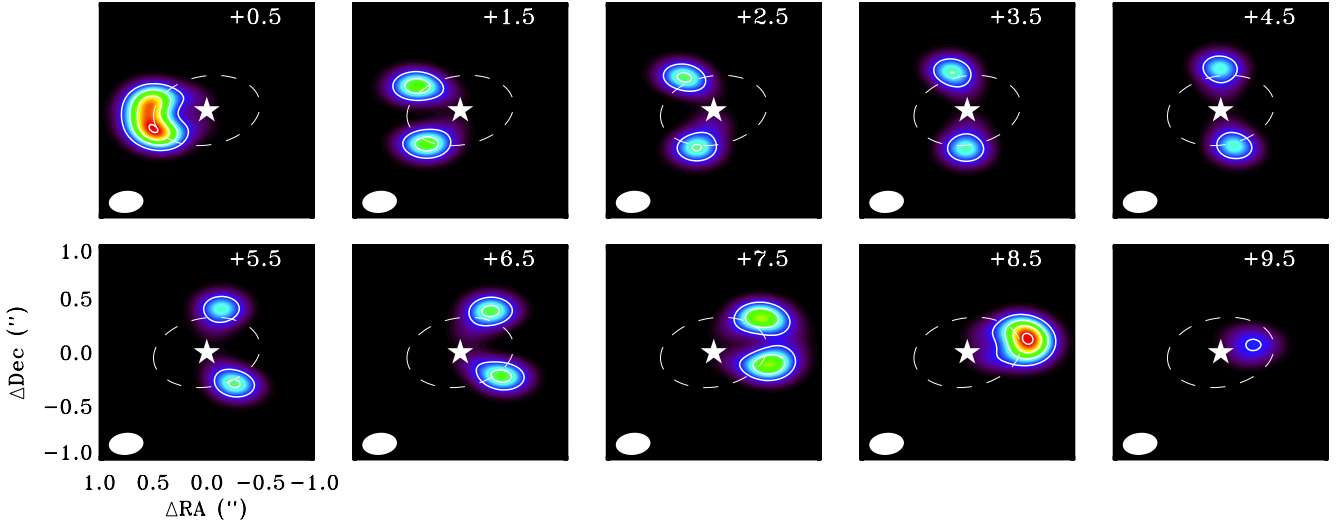
Fig. 10. Results of \text{H}_2\text{CO} abundance modeling: channelmap convolved with the ALMA beam of the observations for Model 1 at 10^{-8} abundance. The 60 AU radius is indicated with a dashed ellipse and the stellar position with a star. The white contours indicate the 20%, 40%, 60%, 80% and 100% of the peak (peak is 212 \text{ mJy beam}^{-1} ).
