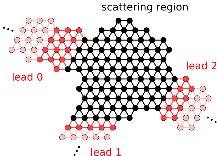
Figure 2. Structure of an exemplary tight-binding system modeled with Kwant. Sites belonging to the scattering region are represented by black dots, sites belonging to one of the three semi-infinite leads by red dots. Each non-zero off-diagonal Hamiltonian element H_{rr'} is shown as a line between site r and site r' . Leads consist of an infinite sequence of interconnected identical unit cells. In this figure, the unit cells of a lead are each drawn in a different shade. Only the first two are shown for each lead.
