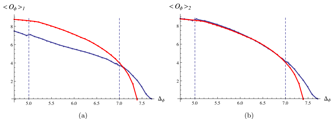
Figure 14. (a): The blue curve represents a particular linear combinations of the series expansion coefficients \langle \mathcal{O}_\phi \rangle_1 = \mathcal{H}_1 + \frac{1}{2}((2\Delta_\Psi + 2) - \Delta_\phi)\mathcal{P}_1 + \frac{1}{2}(\Delta_\phi - 2\Delta_\Psi)\mathcal{P}_3 such that all the resonances cancel out. The red curve included for comparison represents \langle \mathcal{O}_\phi \rangle at \eta_5 = 0 . (b): The serendipitous combination \langle \mathcal{O}_\phi \rangle_2 = \mathcal{H}_1 + \frac{1}{2}e^{-(2\Delta_\Psi - \Delta_\phi)}((2\Delta_\Psi + 2) - \Delta_\phi)\mathcal{P}_1 + \frac{1}{2}e^{-(2\Delta_\Psi + 2 - \Delta_\phi)}(\Delta_\phi - 2\Delta_\Psi)\mathcal{P}_3 that has a remarkable overlap with the \eta_5 = 0 solution at low \Delta_\phi as desired. All parameters are as in figure 10.
