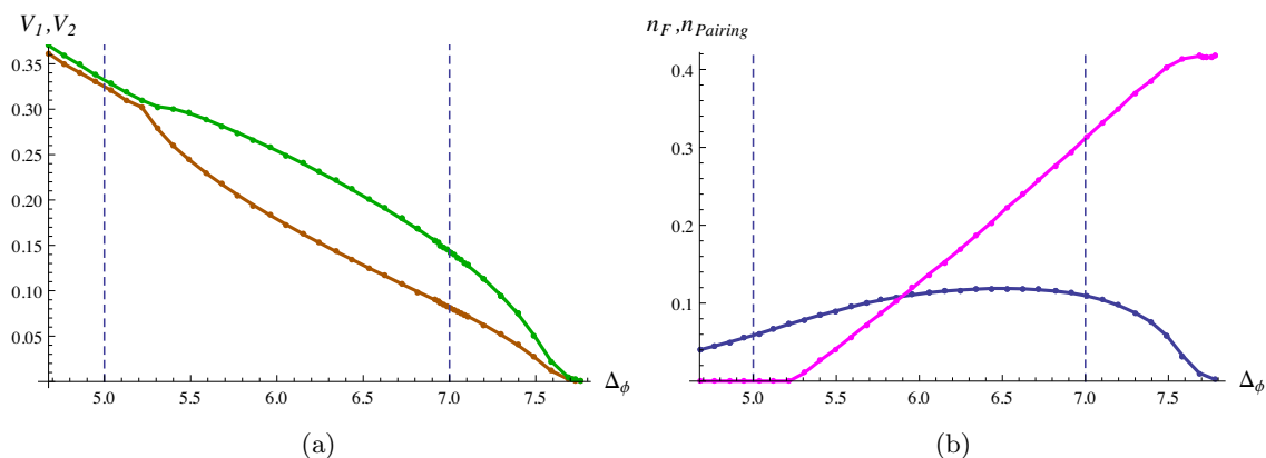
Figure 13. (a): Dependence of the two gaps V_1 (orange) and V_2 (green) on \Delta_\phi in the fully interacting case. (b): Dependence of the total fermionic bulk charge n_F = \int_0^{z_w} qz^2 \langle \psi^\dagger \psi \rangle dz (magenta) and the total “number” of pairs n_{Pairing} = -i\eta_5 \int_0^{z_w} z^3 \langle \bar{\psi} \Gamma^5 \psi \rangle dz (blue) on \Delta_\phi . One can see that while at small scalar conformal dimensions the fermionic bulk charge totally vanishes the number of Cooper pairs in the bulk theory stays finite. All parameters are as in figure 10.
