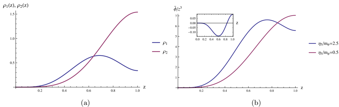
Figure 5. (a): wave function profiles of the fermions at the two Fermi surfaces ( \rho_1, \rho_2 ) ( q\mu = 4.5 , z_w = 1 , m_\psi ). (b) The profiles of the stable solutions of the gap equation \tilde{\phi} = \phi \exp\left(\frac{bx+c}{\gamma_2}\right) (rescaled by z^3 ) for \eta_5/\omega_D = 0.5 , \eta_5/m_\phi = 0.5 and \eta_5/m_\phi = 2.5 . Depending on the coupling the profiles are similar to the fermion wave-functions \rho_1, \rho_2 . In the inset we plot the unstable solution for \eta_5/m_\phi = 2.5 (for the other value of the coupling this mode is exponentially small).
