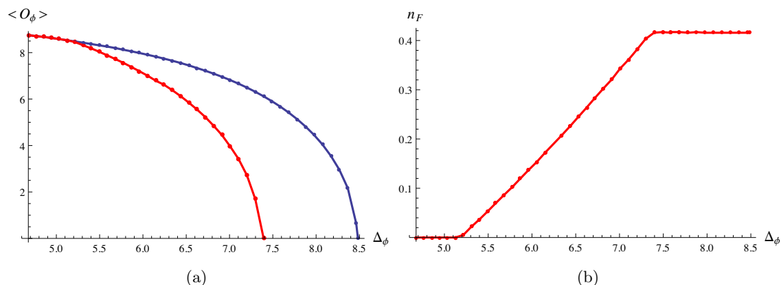
Figure 8. (a): Comparison of the superconducting phase transition in a purely scalar system (blue curve) to the one in a system with fermions at \eta_5 = 0 (red curve). At small conformal dimension there is no difference between the phase curves at all, while for larger dimension we see effects of Bose-Fermi competition. (b): Total fermionic bulk charge as a function of scalar conformal dimension, n_F = \int_0^{z_w} qz^2 \langle \psi^\dagger \psi \rangle dz . Here \mu q = 4.5 , z_w = 1 , q_\phi = 2 , \omega_D = 0.7 .
