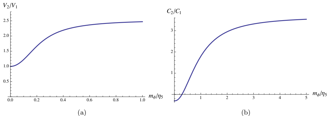
Figure 6. (a): The ratio of the gaps ( V_2/V_1 ) as a function of the inverse coupling m_\phi/\eta_5 (for fixed \eta_5/\omega_D = 0.5 ). The other parameters are as in figure 5. For zero boson mass (or infinite coupling) the gaps have the same size but for non-zero mass (smaller coupling) V_2 is bigger and the ratio converges to the value 2.56. (b): The ratio of the coefficients C_2/C_1 as a function of the inverse coupling.
