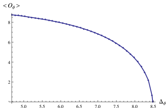
Figure 7. Condensate of a scalar order parameter in the boundary theory as a function of scalar conformal dimension at \mu q = 4.5 , z_w = 1 , q_\phi = 2 .
