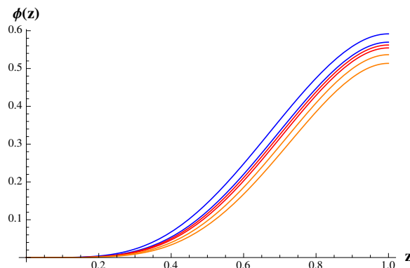
Figure 9. Profiles of the bulk scalar wavefunction \phi(z) for \Delta_\phi = 4.6765 , \Delta_\phi = 4.8541 (two blue curves), \Delta_\phi = 4.9438 , \Delta_\phi = 5.0341 (two red curves, - proximity of the critical point), \Delta_\phi = 5.379 , and \Delta_\phi = 5.4925 (two orange curves). Crossing the critical point \Delta_\phi = 2\Delta_\Psi = 5 does not lead to any singularities in the bulk wavefunction. The other parameters here are \eta_5 = 1 , \mu q = 4.5 , z_w = 1 , q_\phi = 2 , \omega_D = 0.7 .
