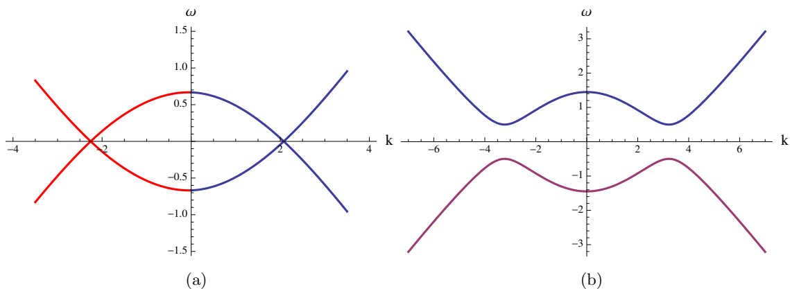
Figure 4. (a): The lower two bands from figure 2 in the Nambu-Gorkov convention (with parameters q\mu = 4.5 , z_w = 1 , m_\Psi = 1 ). (b): Energy spectrum for constant gauge field qA_0 = q\mu = 4.5 and linear fixed scalar profile \phi(z) = z at \eta_5 = 0.25 ( z_w = 1 , m_\Psi = 1 ). The spectrum is gapped at the Fermi surface.
