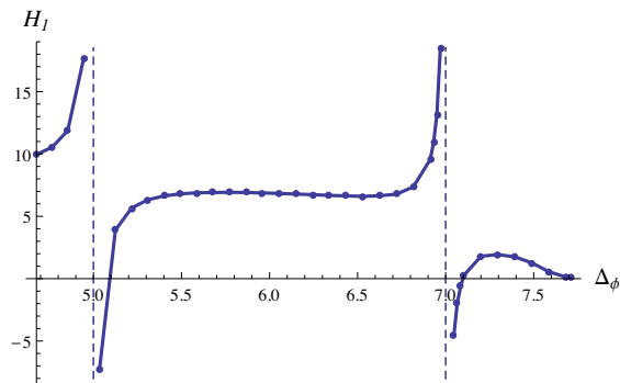
Figure 10. Dependence of the leading homogeneous coefficient in the scalar solution expansion on the conformal dimension of the field. Here \mu q = 4.5 , \eta_5 = 1 , z_w = 1 , q_\phi = 2 , m_\Psi = 1 (so 2\Delta_\Psi = 5 ), \omega_D = 0.7 .
