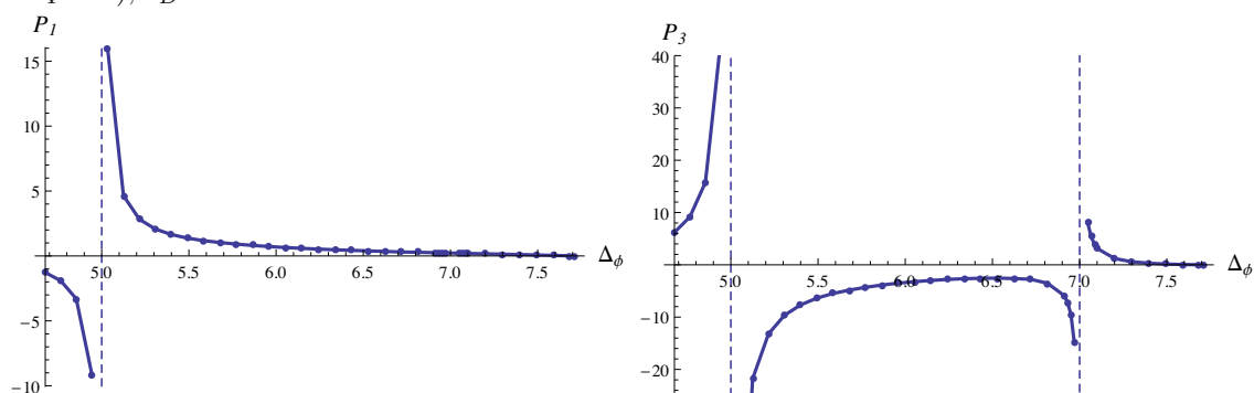
Figure 10. Dependence of the leading homogeneous coefficient in the scalar solution expansion on the conformal dimension of the field. Here \mu q = 4.5 , \eta_5 = 1 , z_w = 1 , q_\phi = 2 , m_\Psi = 1 (so 2\Delta_\Psi = 5 ), \omega_D = 0.7 .
