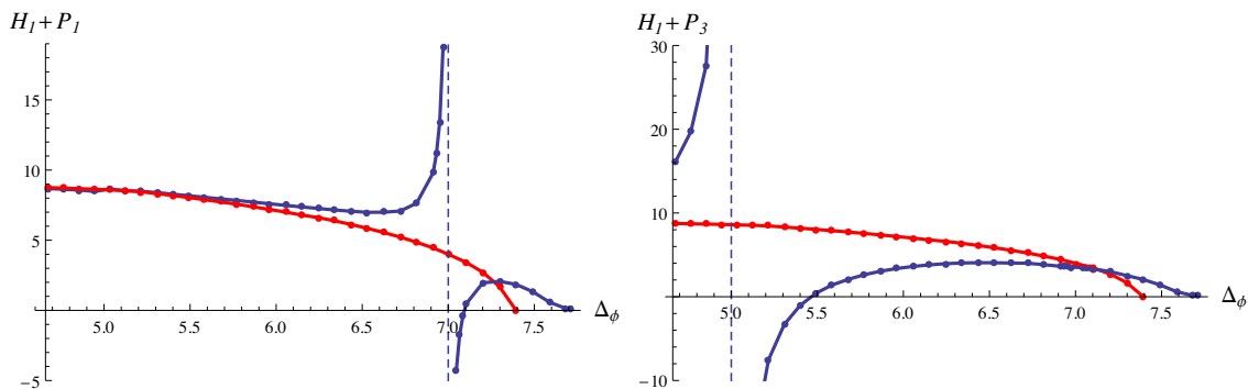
Figure 12. Linear combinations of the series expansion coefficients. Red curve represents the boundary scalar operator condensate \langle \mathcal{O}_\phi \rangle as a function of its conformal dimension in presence of fermions at \eta_5 = 0 (the same as the red curve on figure 8). The blue curve represent the linear combination \mathcal{H}_1 + \mathcal{P}_1 on the left plot, and \mathcal{H}_1 + \mathcal{P}_3 on the right one. Resonances in \mathcal{H}_1 and \mathcal{P}_1 precisely cancel each other at \Delta_\phi = 2\Delta_\Psi , and so do resonances in \mathcal{H}_1 and \mathcal{P}_3 at \Delta_\phi = 2\Delta_\Psi + 2 . All parameters are as in figure 10.
