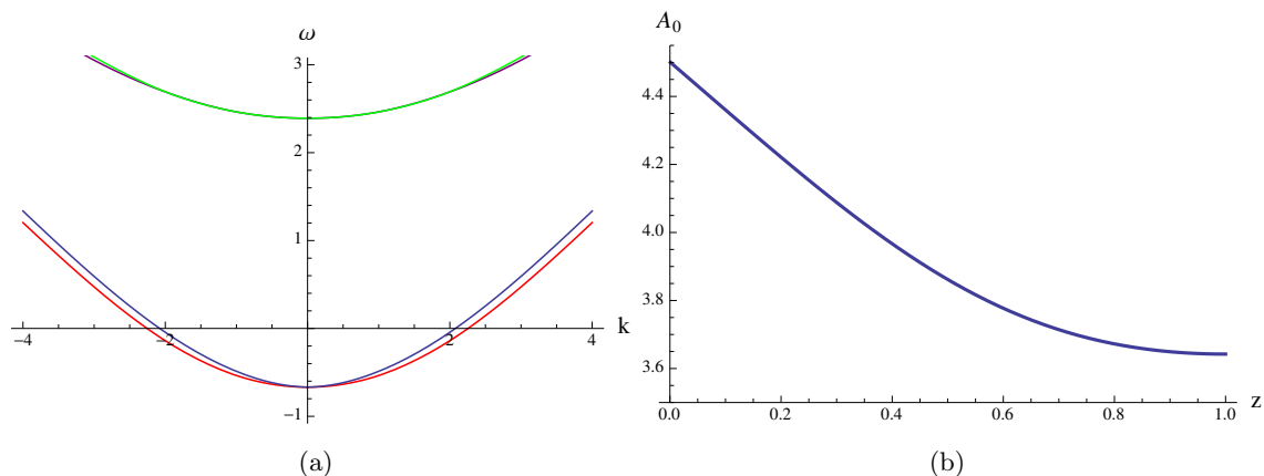
Figure 2. (a): Fermionic spectrum in the self-consistent solution of the fermion+gauge field system at q\mu = 4.5 , z_w = 1 and m_\Psi = 1 . The red and blue curves represent the modes with positive and negative eigenvalues of \hat{k}_i \Gamma^i \Gamma^0 respectively. (b): The profile of the gauge field sourced by the fermions.
