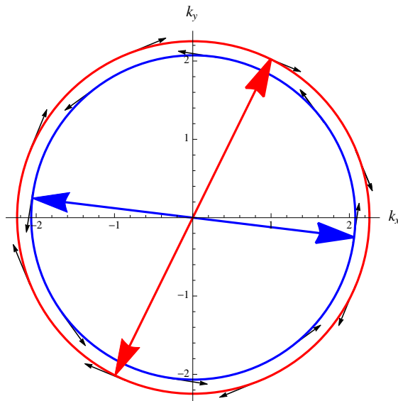
Figure 3. The two Fermi surfaces and the BCS pairing for the same parameters as in figure 2. The arrows indicates the direction of the spin of the modes. The pairing happens between opposite spins.
