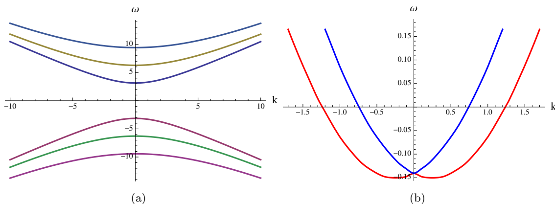
Figure 1. (a): Fermionic spectrum in the AdS-hardwall background at zero chemical potential z_w = 1 and m_\Psi = 1 (b): Spectrum of fermions with unit mass (and z_w = 1 ) in the presence of externally applied electric field qA_0(z) = 4.5 - 2z (without backreaction) . We can observe that degeneracy of the two spin states is resolved, and state of a minimal energy is at non-zero momentum. The red and blue curves correspond to positive u_+(k) and negative u_-(k) modes respectively. (When the electric field is self-generated by the fermions the effect is smaller, see figure 2(a))
